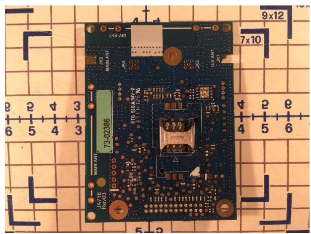
Module - Bottom View
