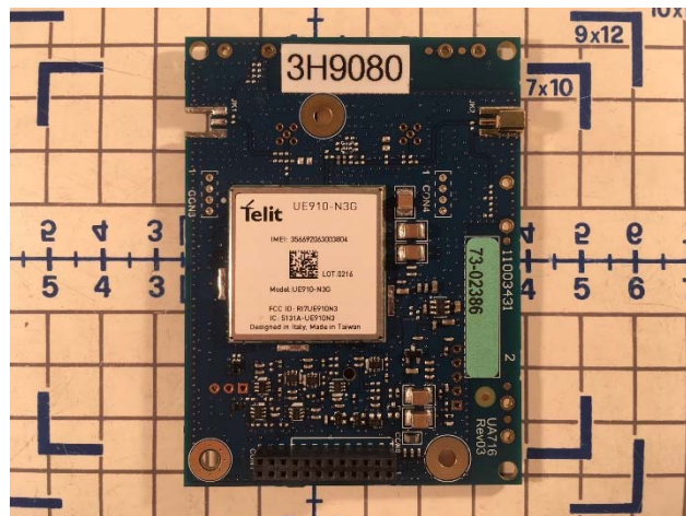
Module - Top View
