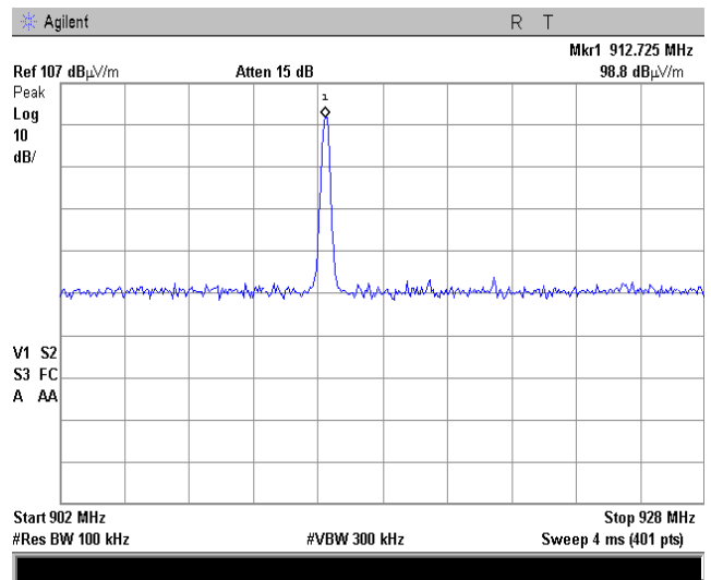
Plot 7.6.2 Radiated emission measurements at the low carrier frequency
