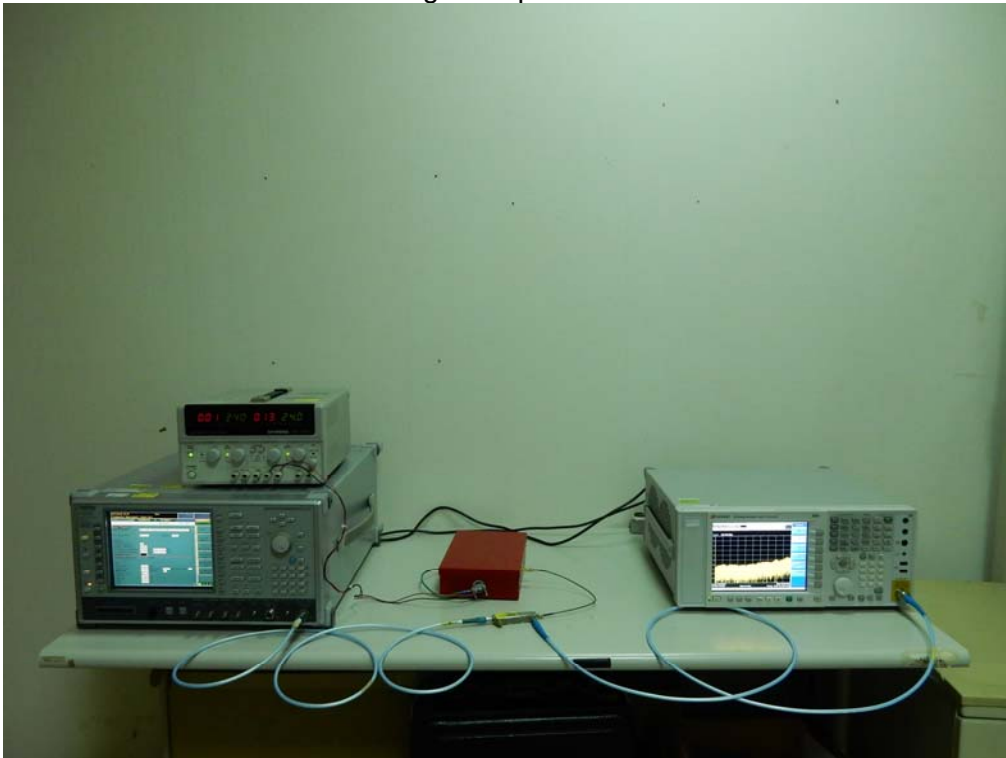
Front View of High Frequnc Conducted Test
