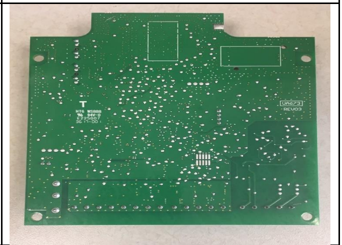
Main PCB - Top View without shielding
