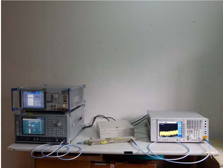
Front View of High Frequenc Conducted Test
