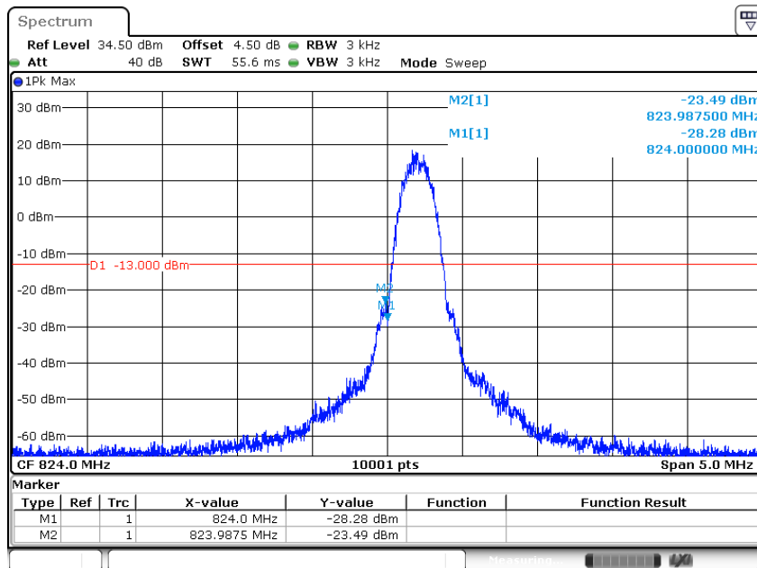
Figure Channel 128 (824.20MHz)
