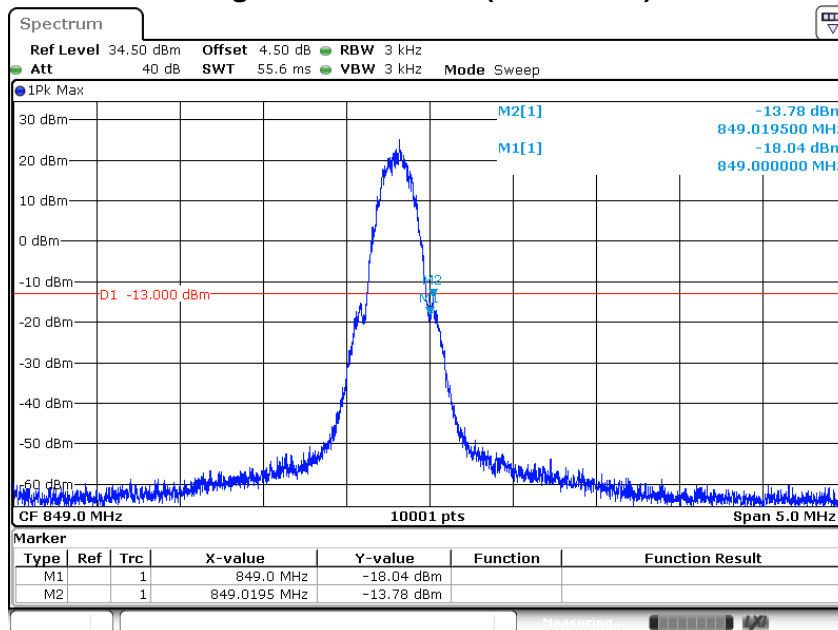
Figure Channel 251 (848.80MHz)
