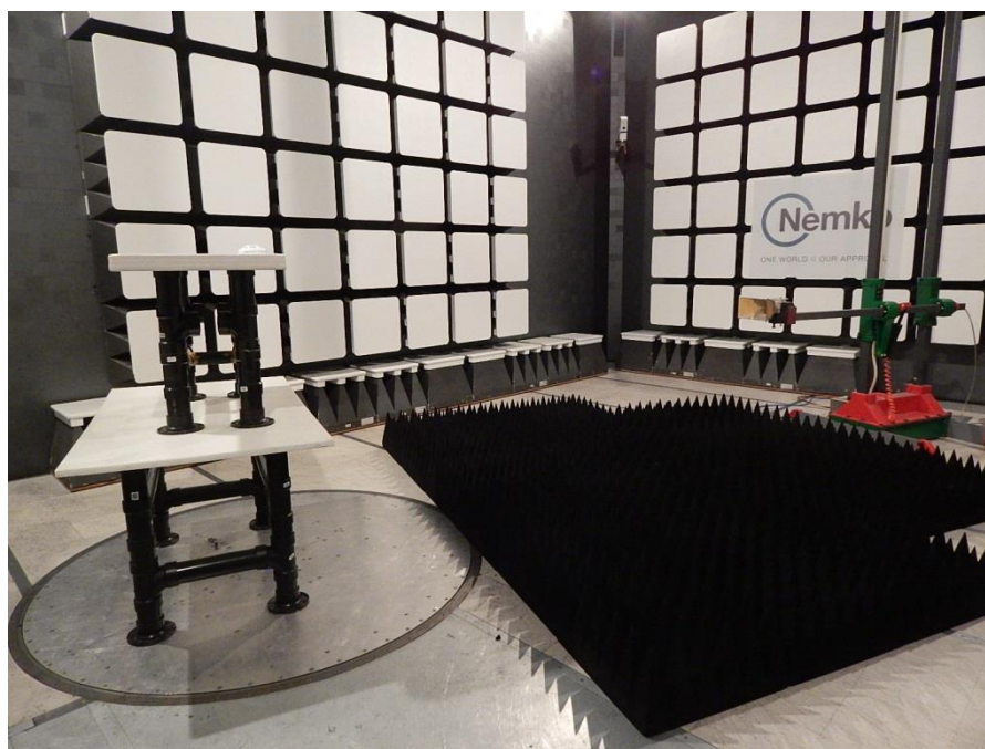
Figure Error! No text of specified style in document.-2: Emissions setup photo – above 1 GHz
