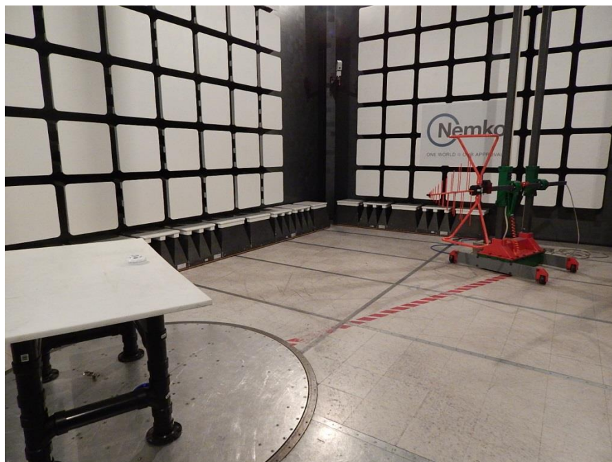
Figure Error! No text of specified style in document.-1: Emissions setup photo – 30 to 1000 MHz
