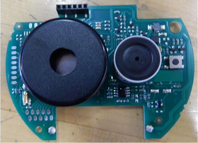
Figure 1-2: Main PCB top view
