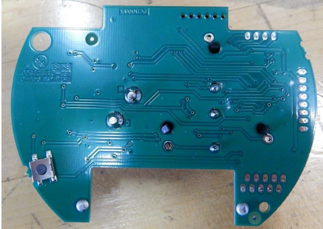
Figure 1-3: Main PCB bottom view
