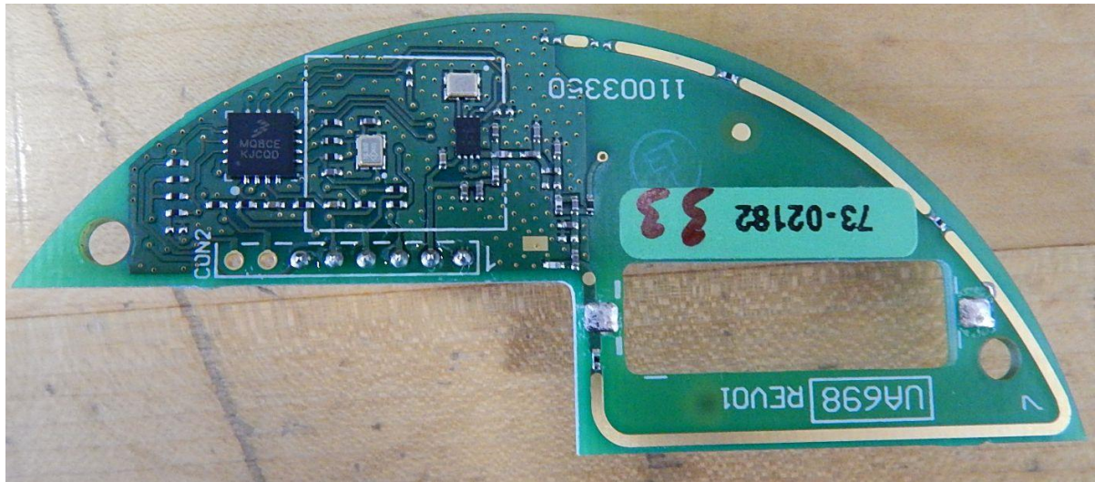
Figure 1-4: RF PCB top view
