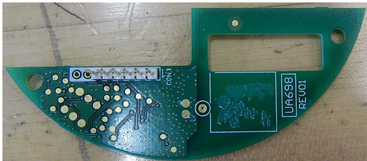
Figure 1-5: RF PCB bottom view
