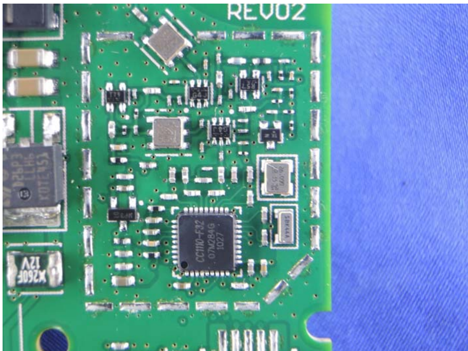
(26) EUT Photo
