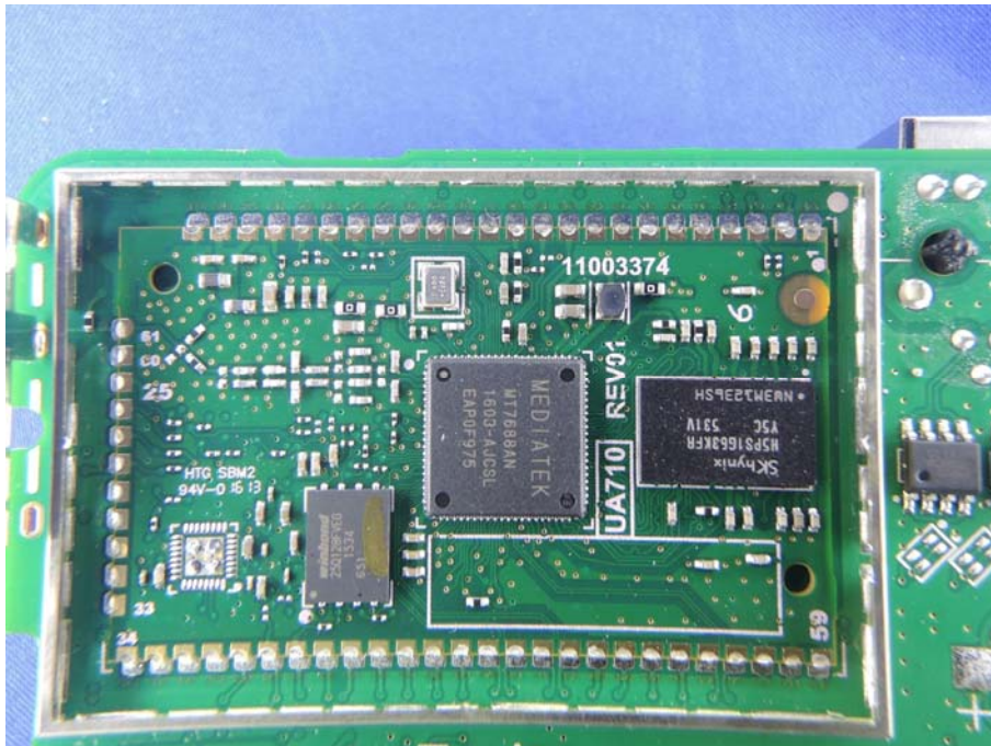
(22) EUT Photo
