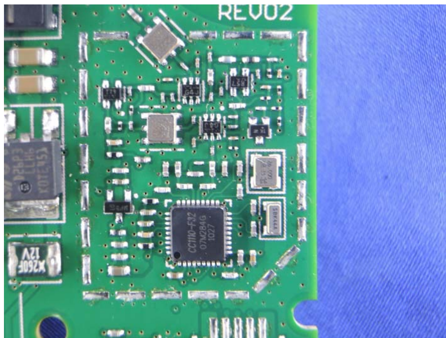
(26) EUT Photo
