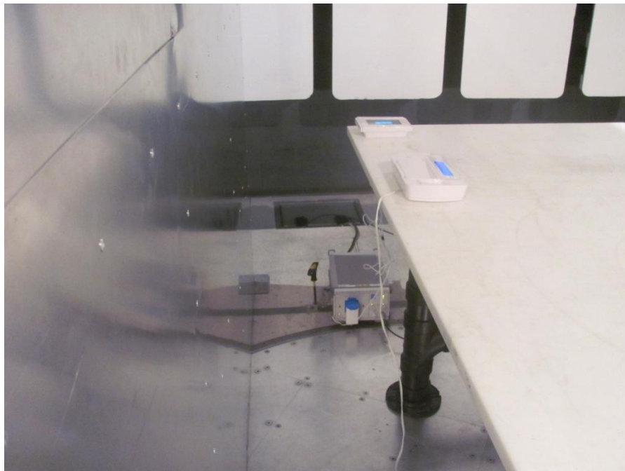
Conducted emissions setup
