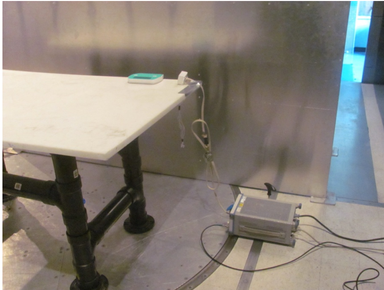
AC power line conducted emissions
