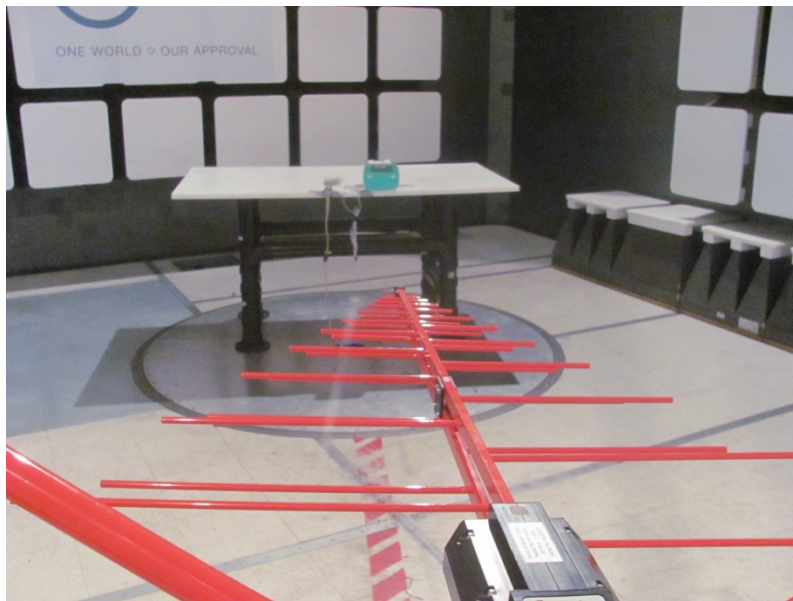
Radiated emissions setup
