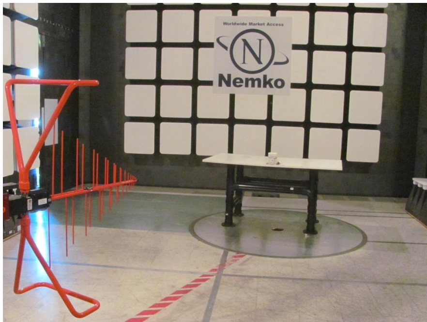
Radiated emissions setup
