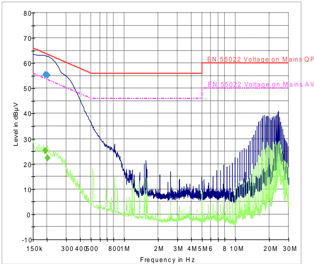
CISPR 22 Mains Conducted FCC_LISN
