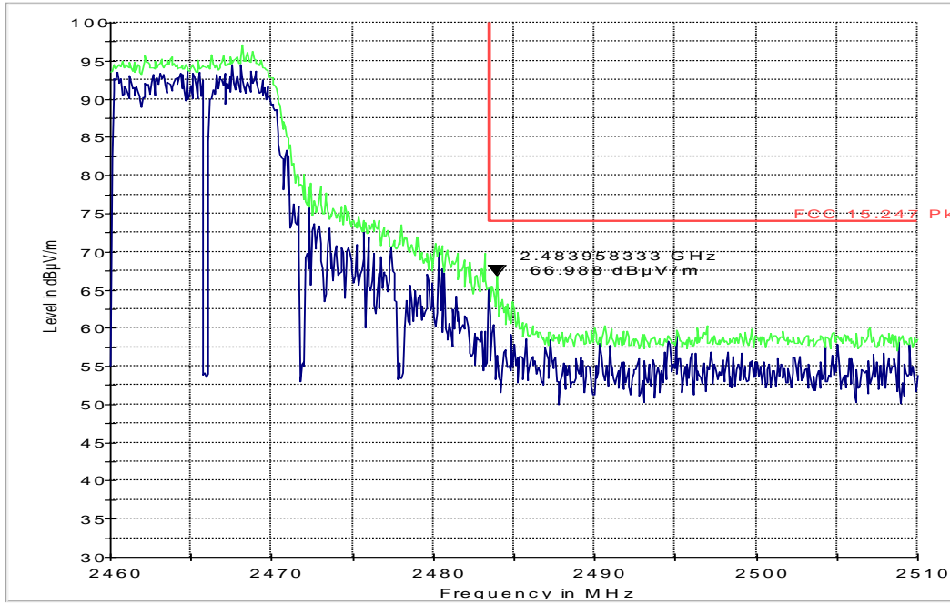
FCC 15.247 HBE Pk 3m
