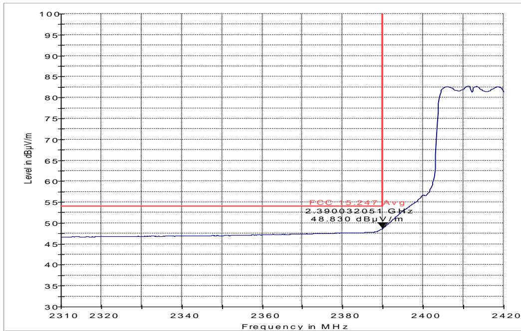
FCC 15.247 LBE Avg 3m
