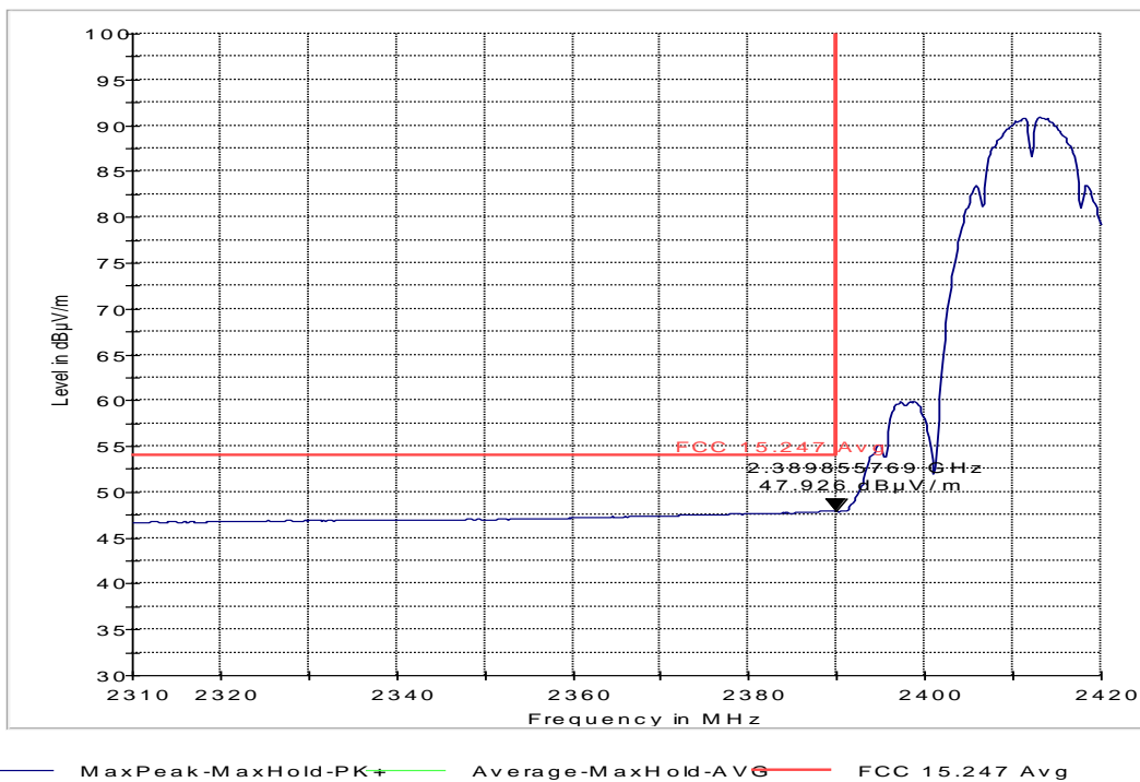
FCC 15.247 LBE Avg 3m
