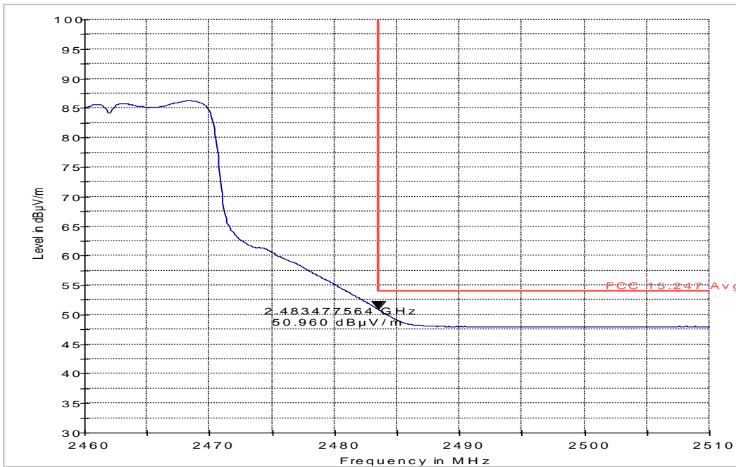
FCC 15.247 HBE Avg 3m
