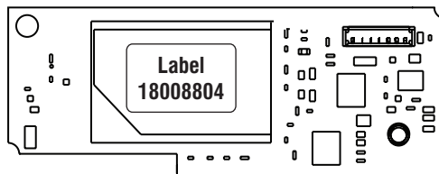
The label is to be located on the top of the unit (PCB) as shown above in actual size
