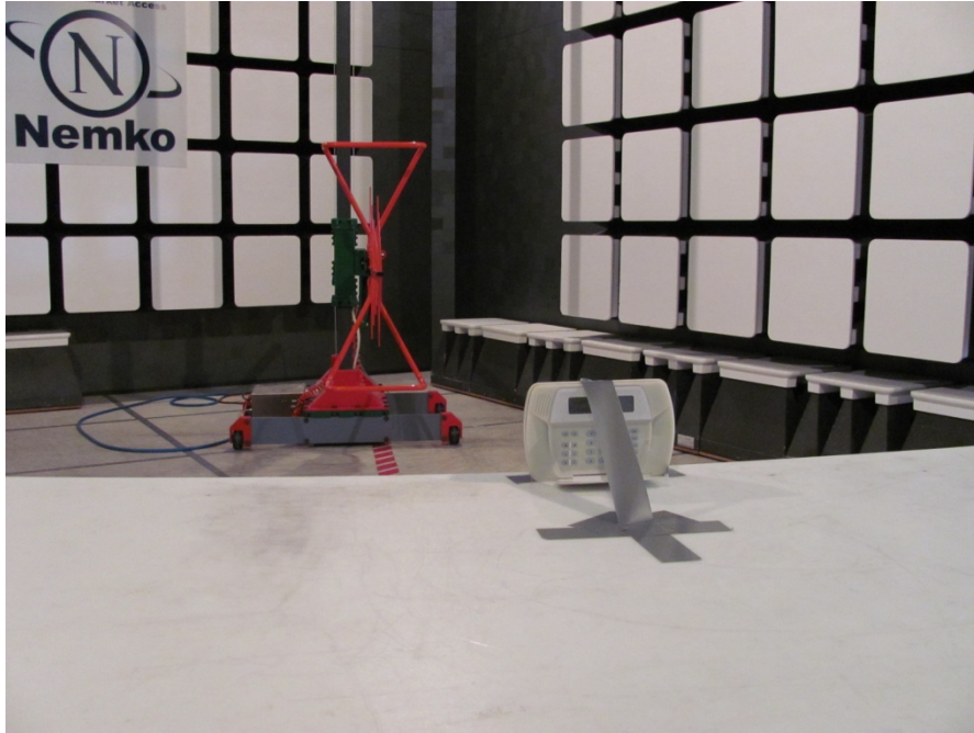
Photo 1: Radiated emissions setup
