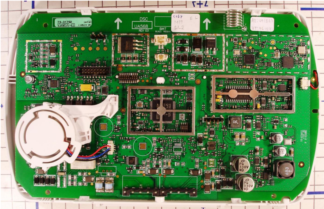
SCW9057(D)(G)(I)(-SM)-433 UA568 Rev 03 PCB top view (RF shields OFF)
