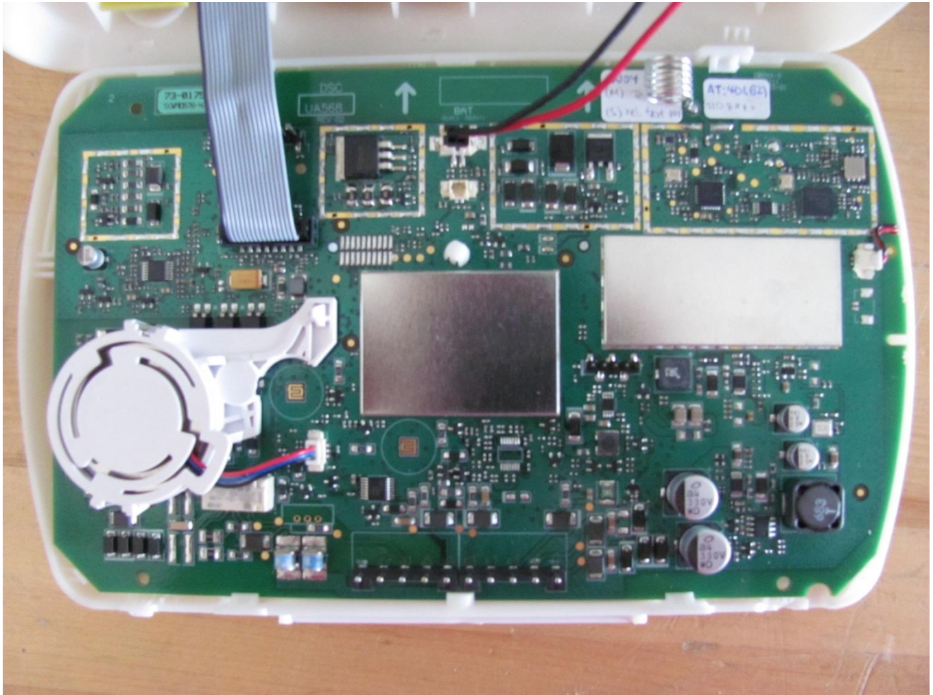
SCW9057(D)(G)(I)(-SM)-433 UA568 Rev 03 PCB top view (RF shields ON)
