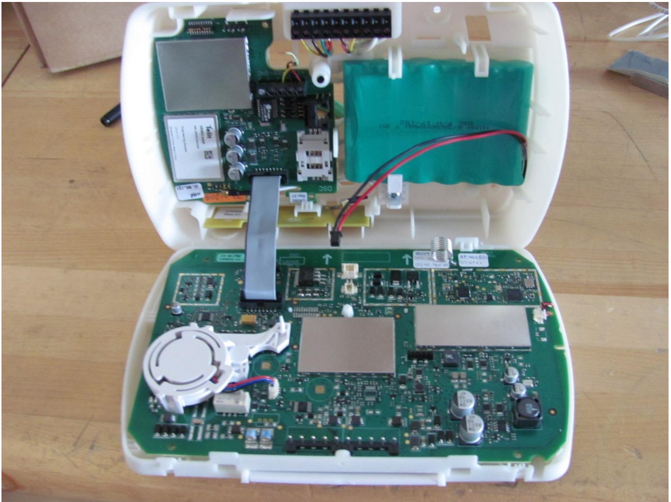
SCW9057(D)(G)(I)(-SM)-433 inside view
