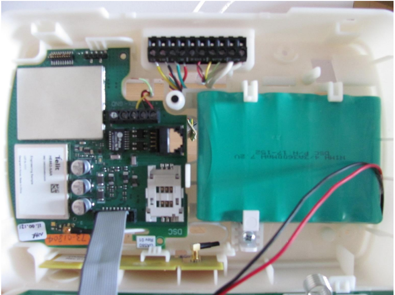
SCW9057(D)(G)(I)(-SM)-433 inside view – alternate communicator board
