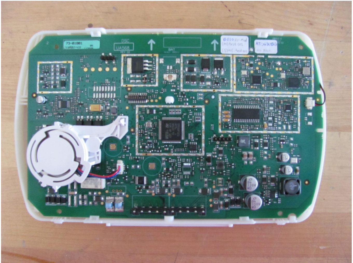
SCW9057-433 UA568 Rev 03 PCB top view
