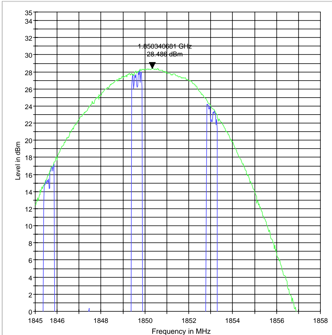
EIRP 1900 L
