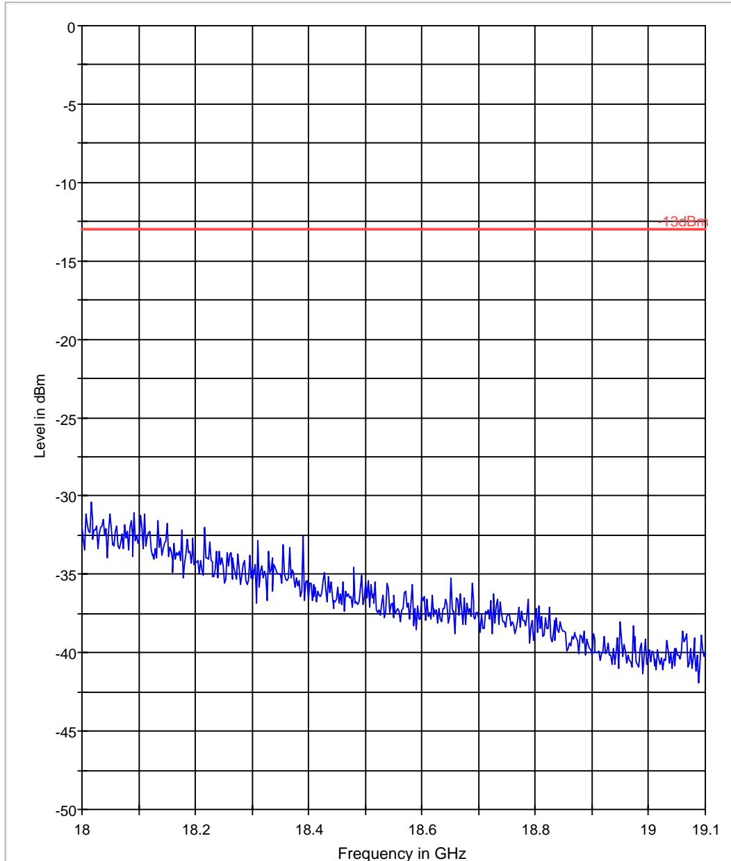
FCC 24 18-19.1GHz
