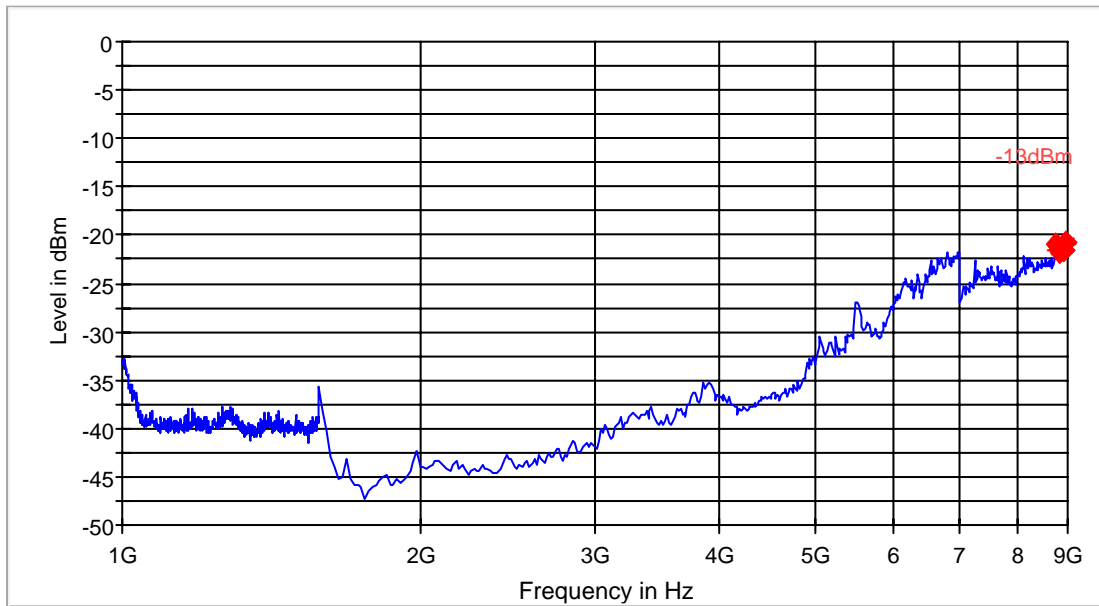
FCC 22 1-9GHz
