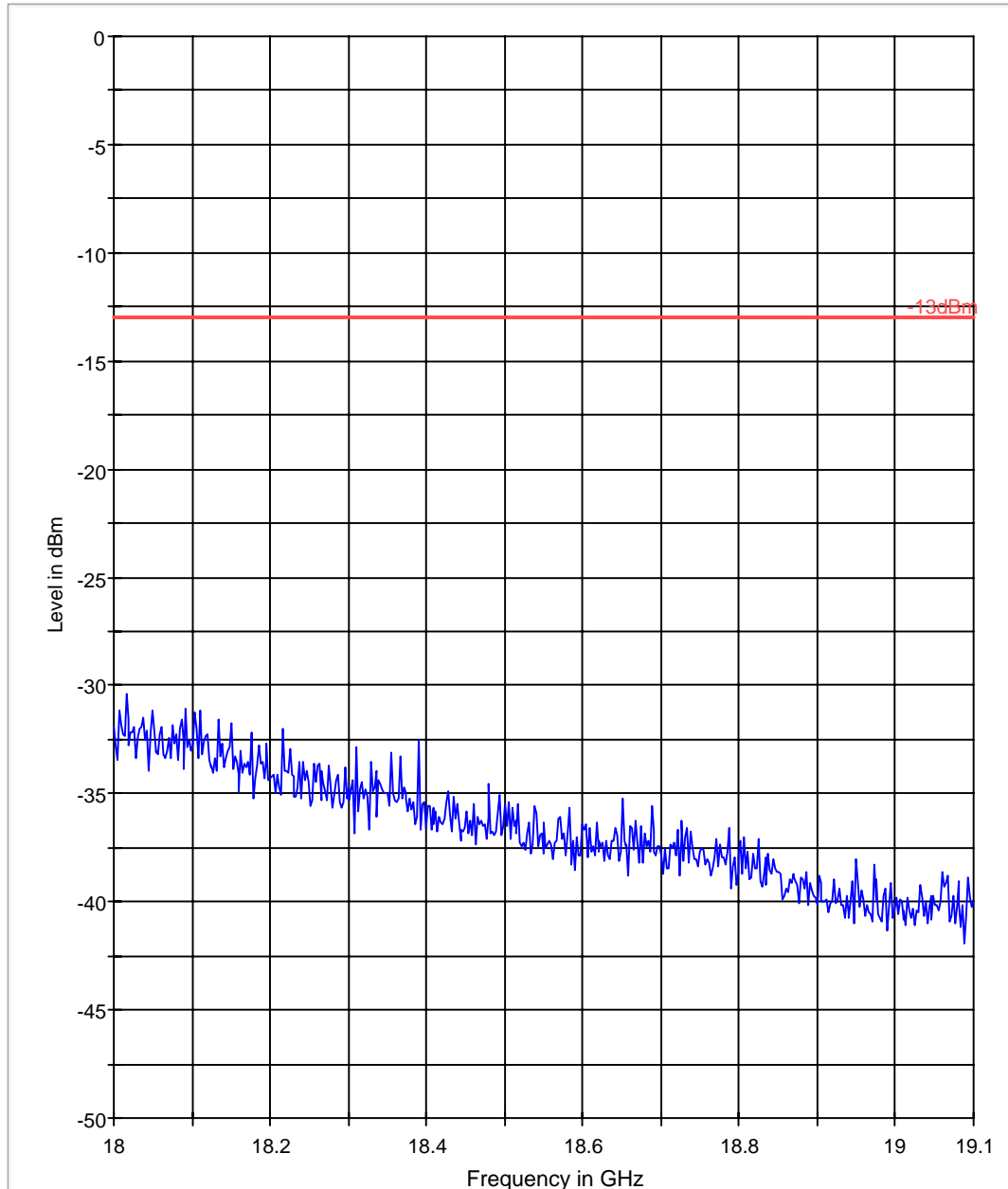
FCC 24 18-19.1GHz
