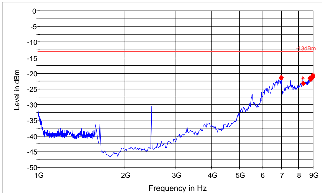
FCC 22 1-9GHz
