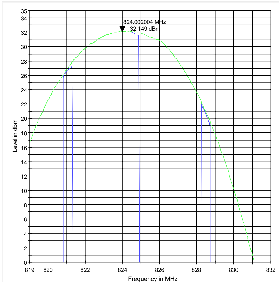
ERP 850 L
