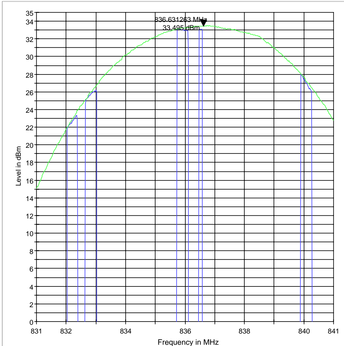
ERP 850 M
