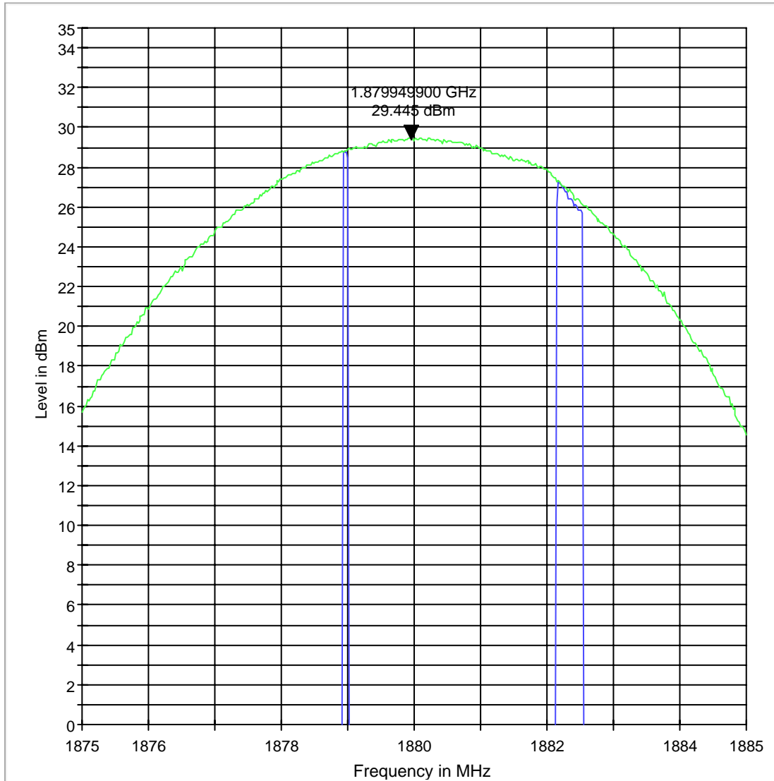
EIRP 1900 M
