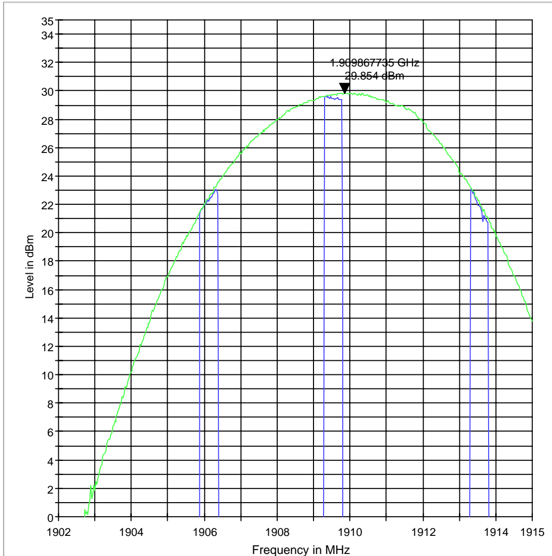
EIRP 1900 H
