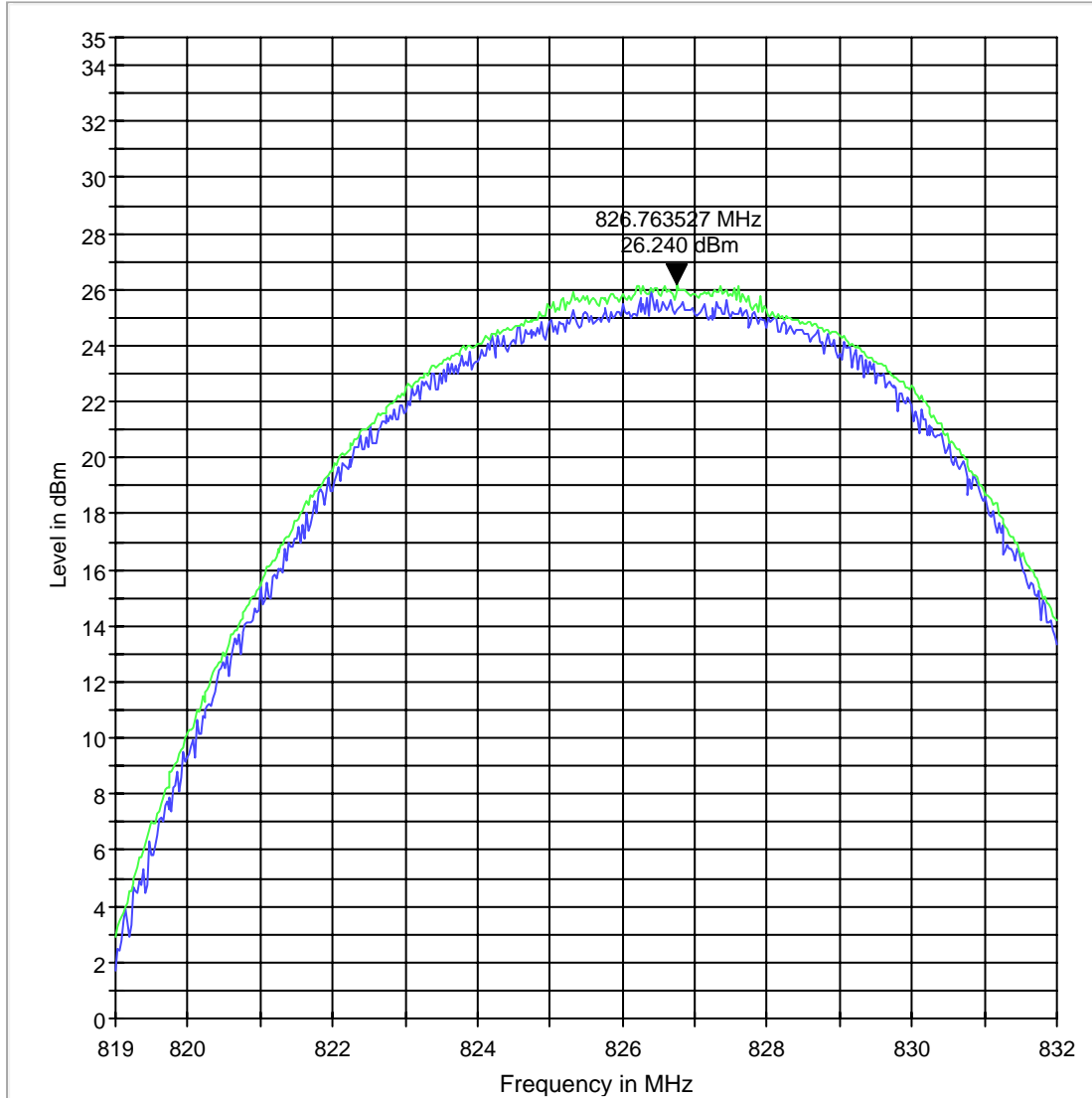
ERP 850 L
