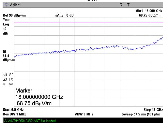
Plot 8.4.14 Radiated emission measurements in 6500 - 18000 MHz range
