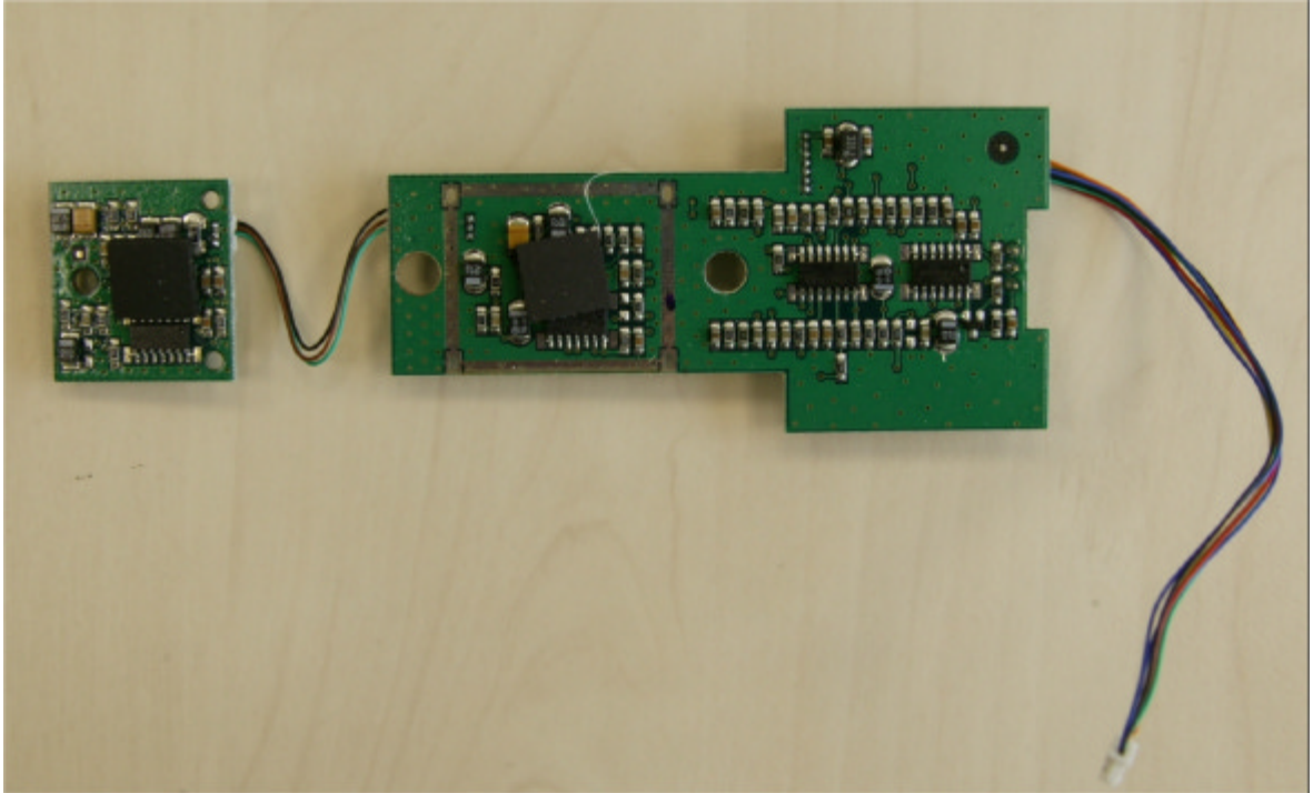
Photograph No.6 Second side of the auxiliary circuits PCB
