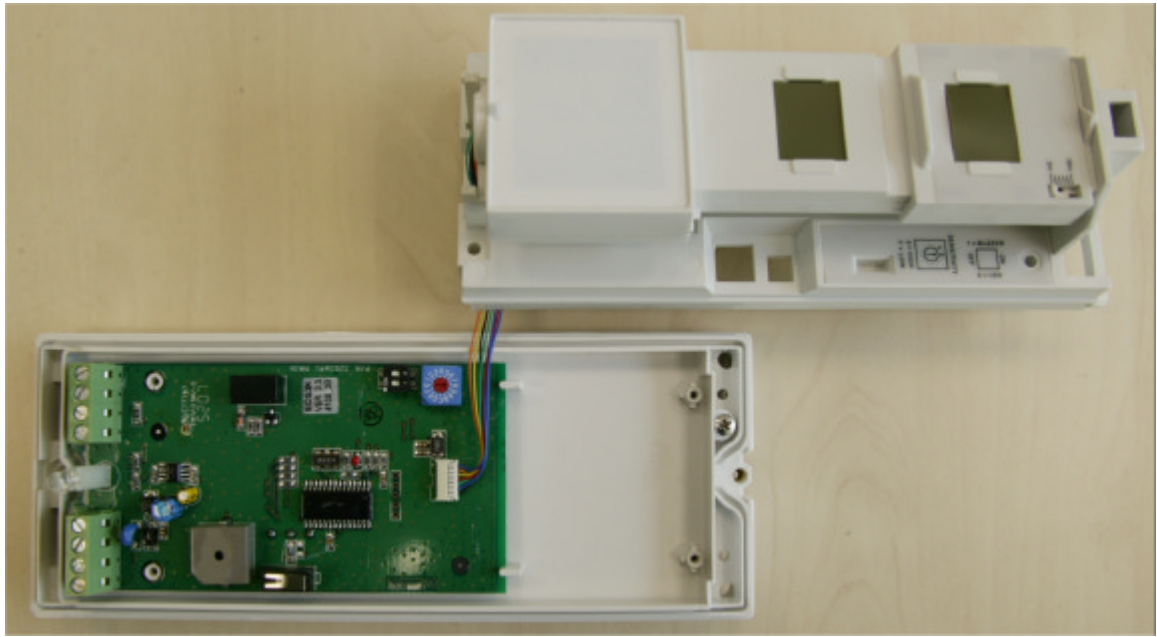
Photograph No.2 Detector internal view with main PCB front view and removed auxiliary circuits
