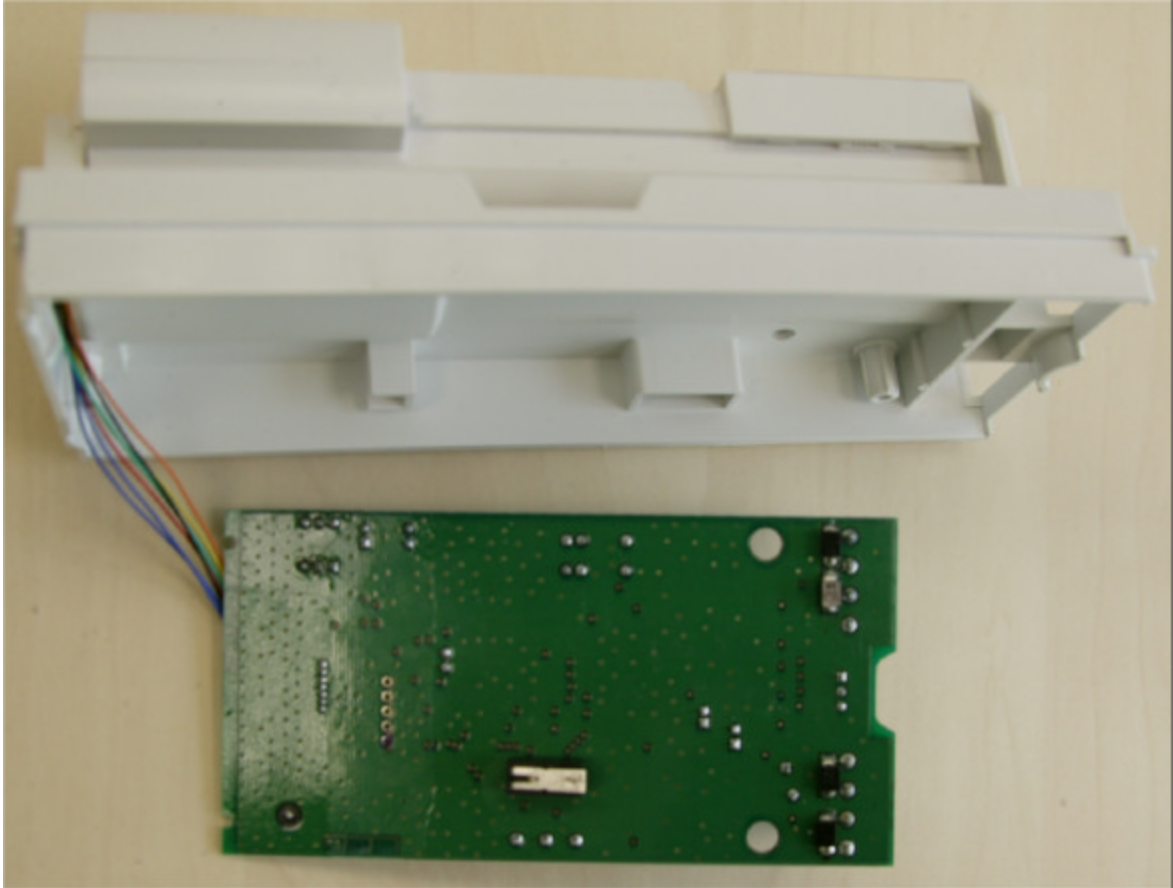
Photograph No.3 Main PCB second side view
