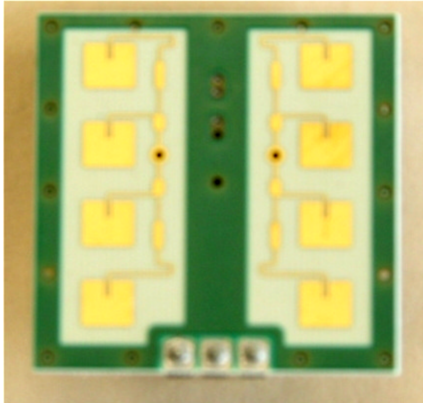
Photograph No.7 RF module front view
