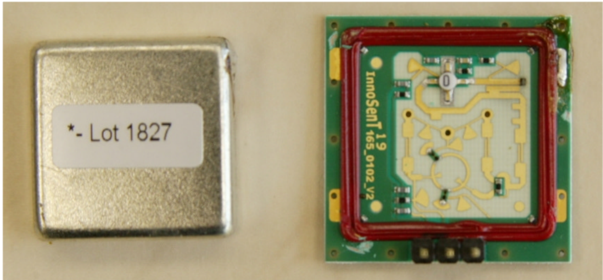
Photograph No9 RF PCB without shielding
