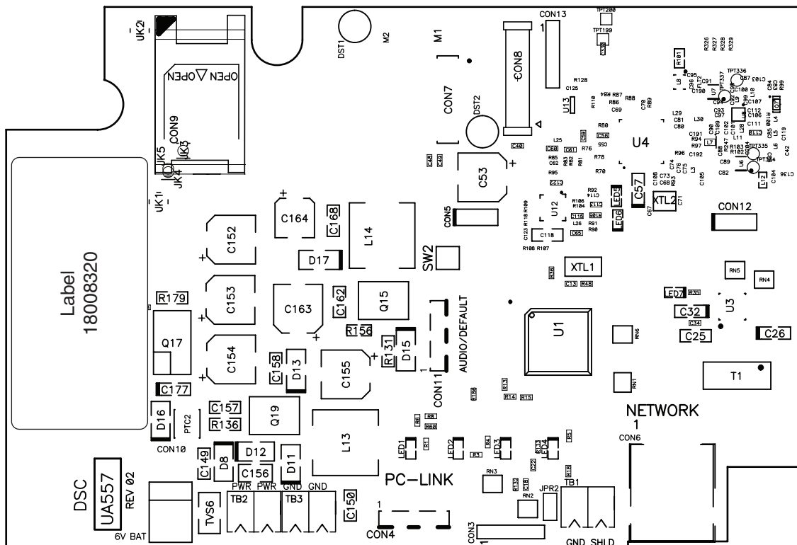
Top of the PCB showing the label location (actual size)
