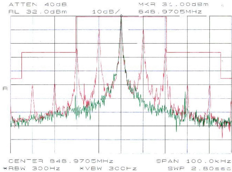
Plot #3: Highest Channel (848.97 MHz) Emission Mask
