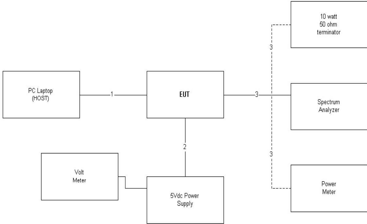
Figure 1. Test Configuration
