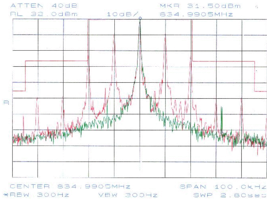
Plot #2: Middle Channel (834.99 MHz) Emission Mask
