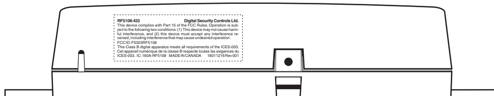
Side of the unit showing placement of label (Actual size)
