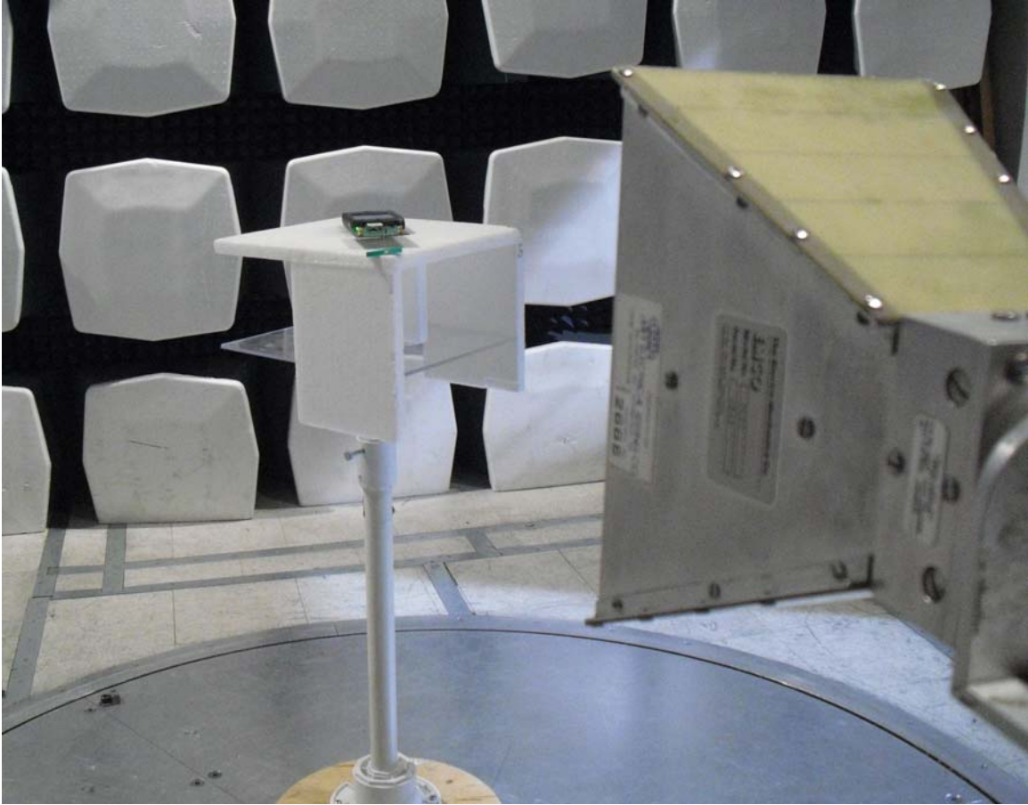
Photograph 4. Bandedge Test Setup PCB 2 dBi
