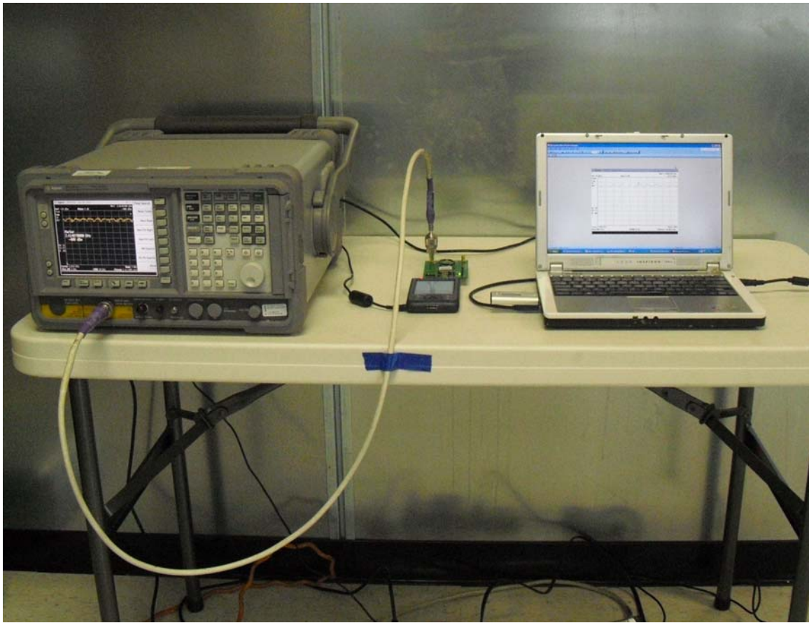
Photograph 1. 6 dB BW Test Setup, Conducted Output Power Test Setup, PSD Test Setup
