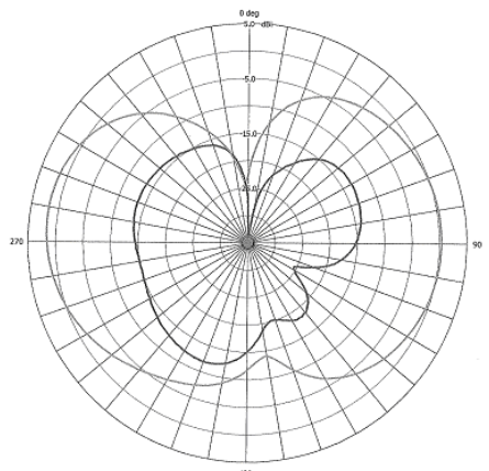
Elevation Plane Phi = 90 2.45 GHz
