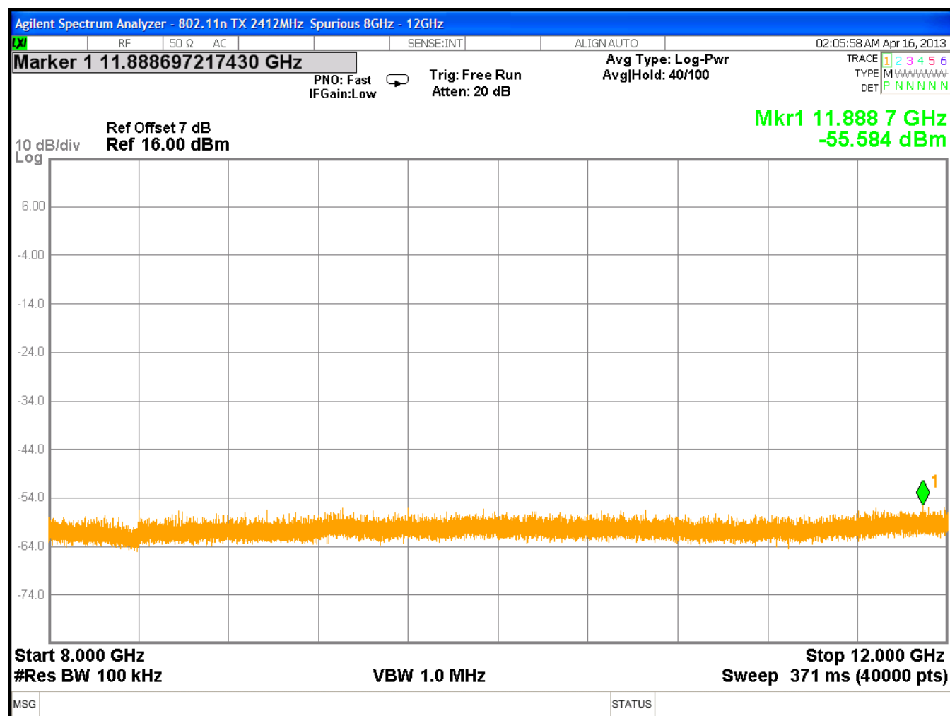
Figure 81: Conducted Spurious Emissions, 2412MHz, 6.5Mbps, 8 - 12GHz
