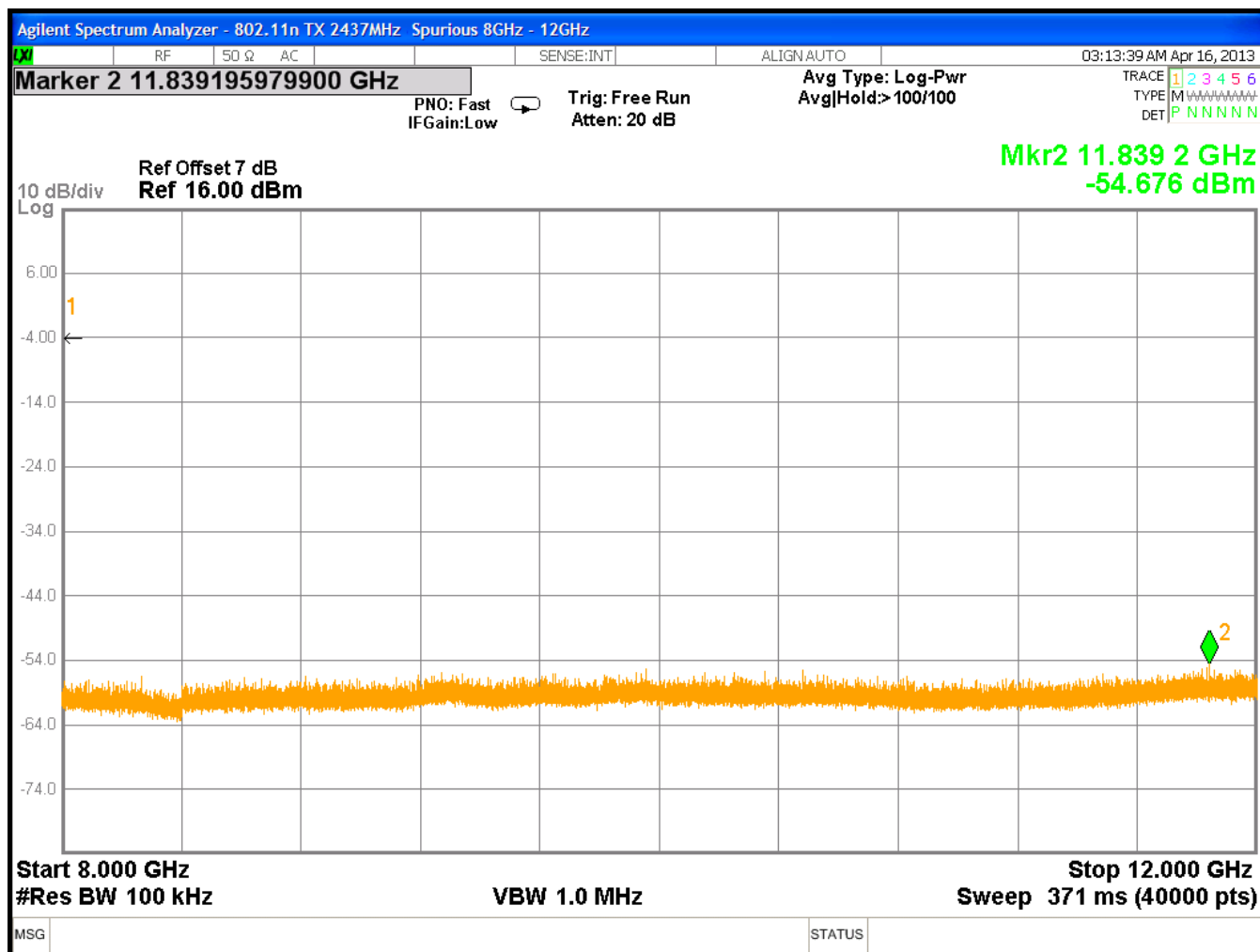
Figure 88: Conducted Spurious Emissions, 2437MHz, 6.5Mbps, 8 - 12GHz
