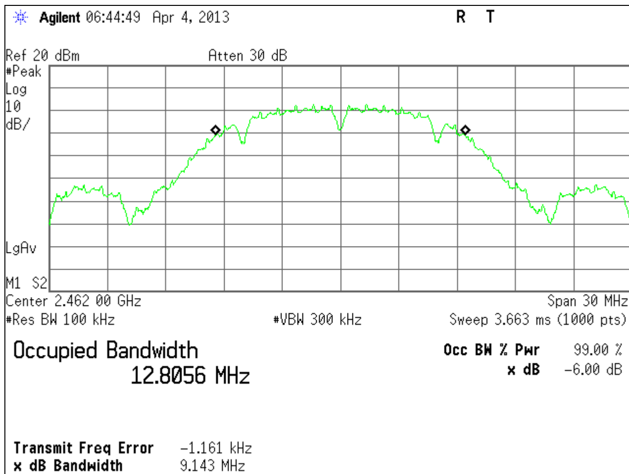
Figure 13: Occupied Bandwidth, 802.11b, 1Mbps, 2462MHz
