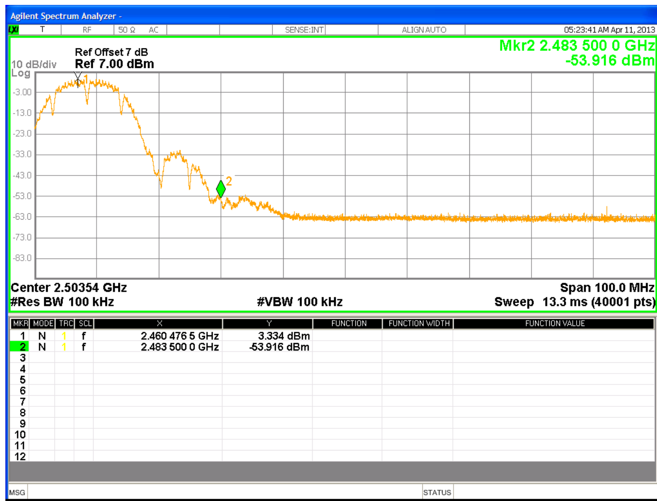
Figure 103: Upper Band-edge, 2462MHz, 802.11b, 1Mbps
