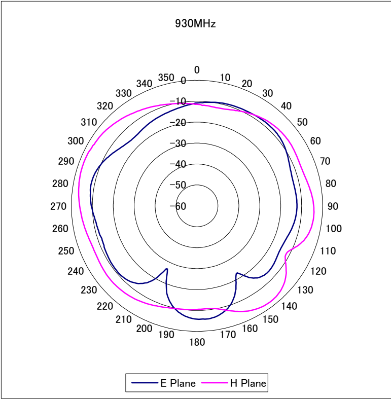
127E8000 2D Pattern[dBi] X-Y
