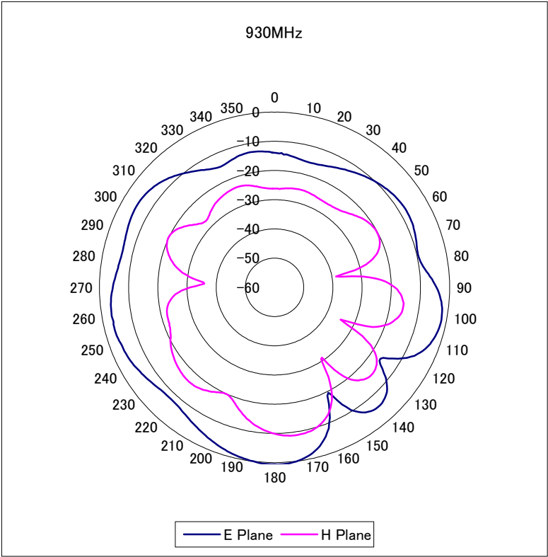
127E8000 2D Pattern[dBi] X-Z
