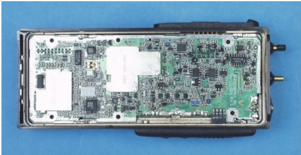
Circuit, Top
