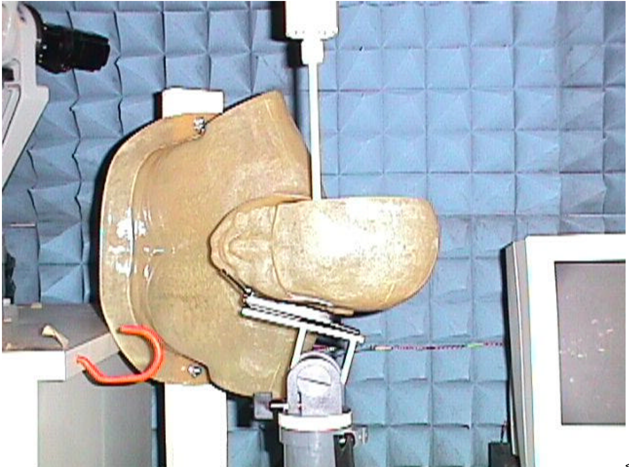
< Head Left Ear SAR Measurement – Overview >
