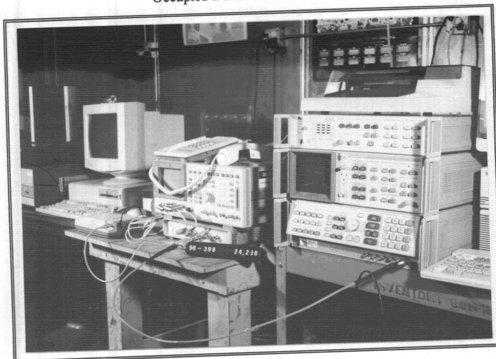
Occupied Bandwidth Test Setup
