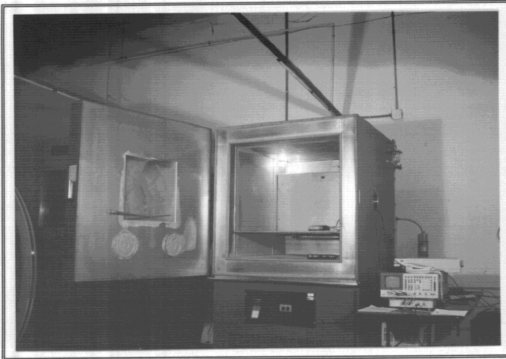
Frequency Stability Test Setup - Temperature Variation
