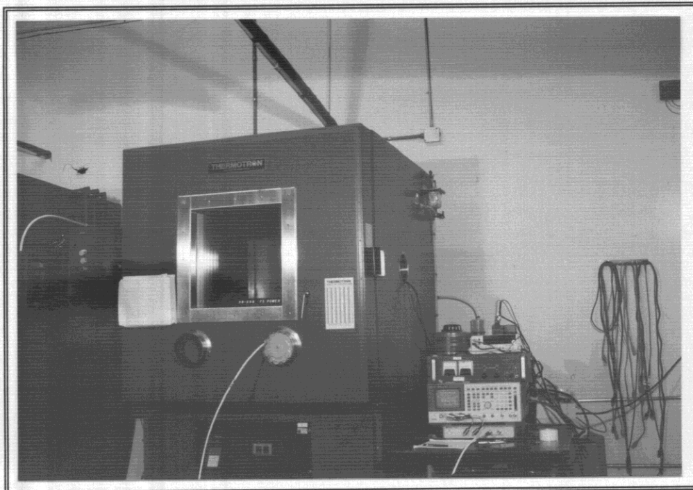
Frequency Stability Test Setup - AC and DC Power Variation
