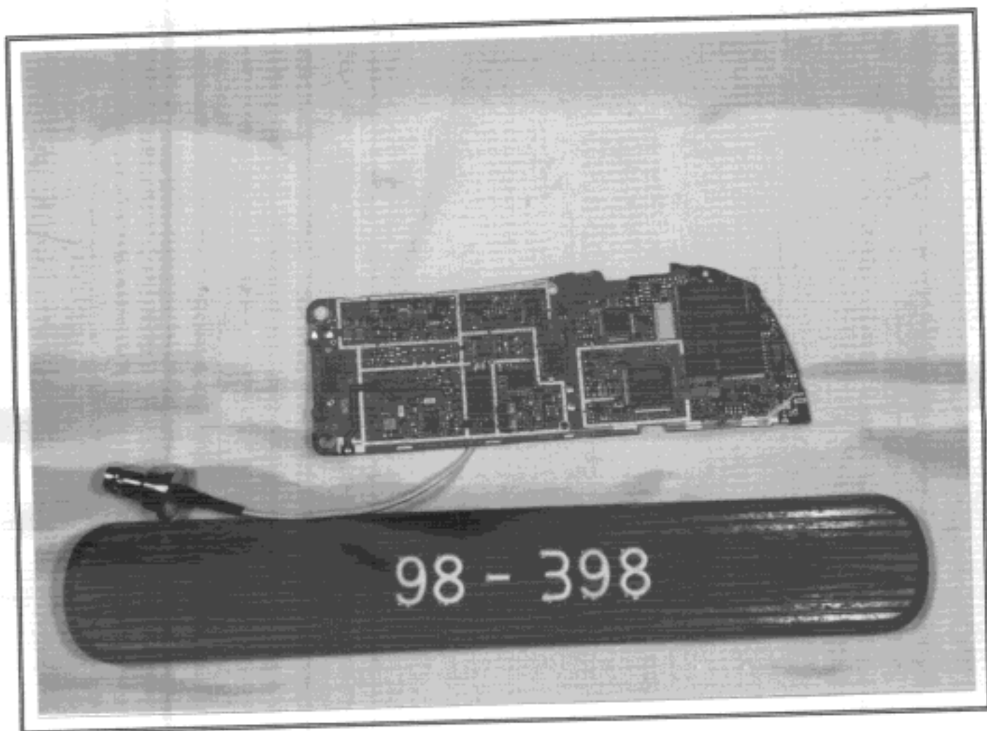
RF Assembly - Top View (Without Shields)
