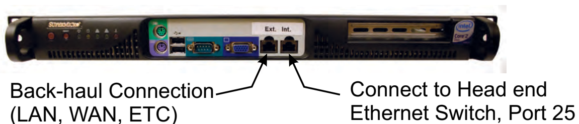
Figure 28 BGW Installation, Ethernet Connections
