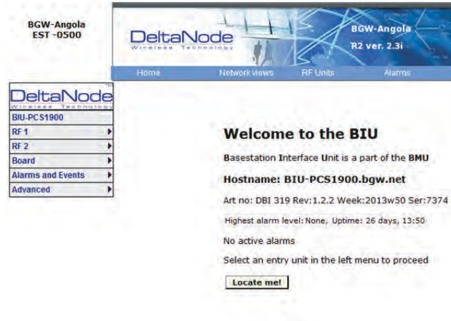
Figure 68 BIU Welcome Screen
