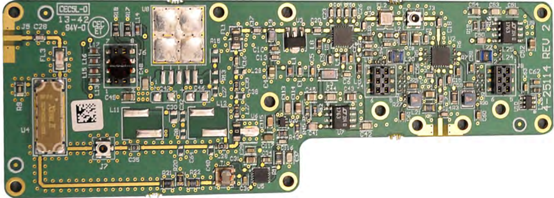
Upconverter Board 3-25113-2 front view
