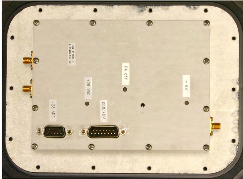
Power Amplifier 3-25406 top view
