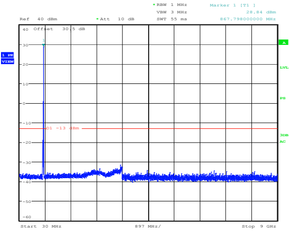
Plot 8.4-65: Spurious emissions Regular + power amplifier Downlink 800 MHz C4FM modulation 868.99375 MHz
