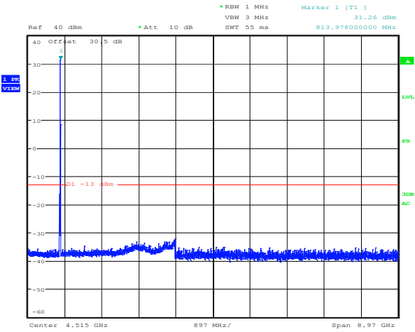
Plot 8.4-33: Spurious emissions Regular + power amplifier Uplink 800 MHz C4FM modulation 815 MHz
