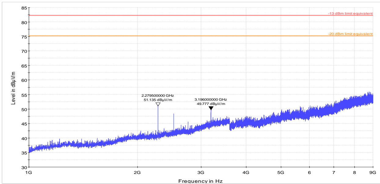
Plot 8.4-78: Radiated spurious emissions Regular + power amplifier Uplink 700 MHz
