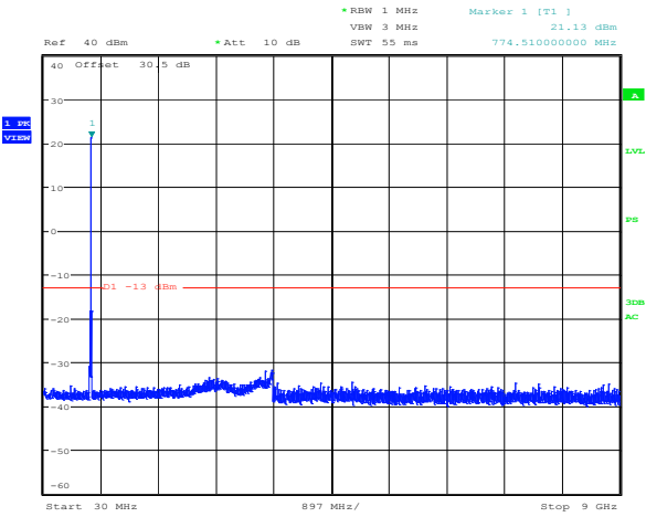
Plot 8.4-9: Spurious emissions Regular + power amplifier Downlink 700 MHz C4FM modulation 774.99375 MHz
