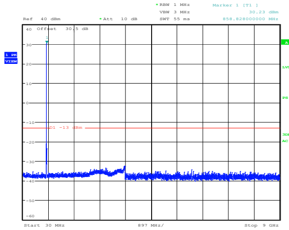
Plot 8.4-58: Spurious emissions Regular + power amplifier Downlink 800 MHz CQPSK modulation 860 MHz
