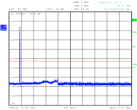
Plot 8.4-25: Spurious emissions Regular + power amplifier Uplink 800 MHz C4FM modulation 806.00625 MHz
