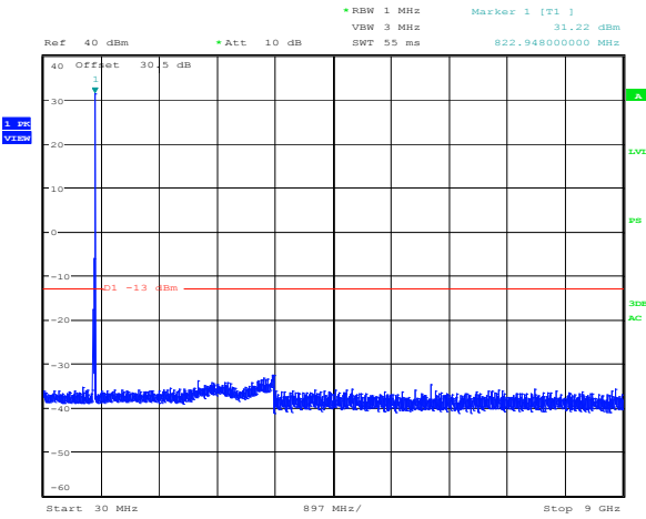
Plot 8.4-45: Spurious emissions Regular + power amplifier Uplink 800 MHz LSM modulation 823.99375 MHz
