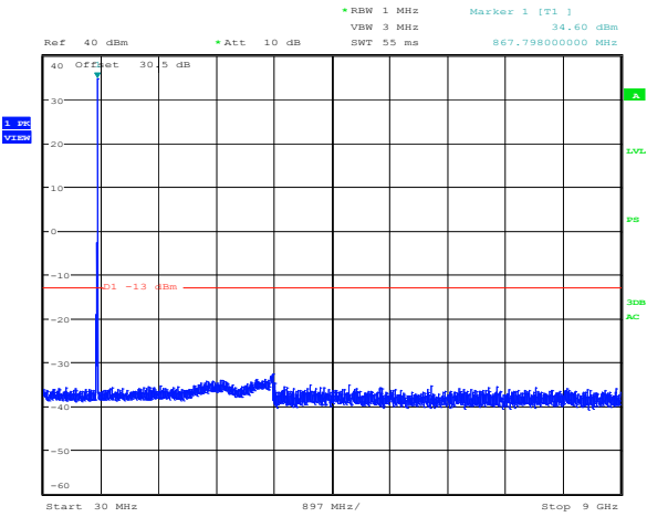
Plot 8.4-69: Spurious emissions Regular + power amplifier Downlink 800 MHz LSM modulation 868.99375 MHz
