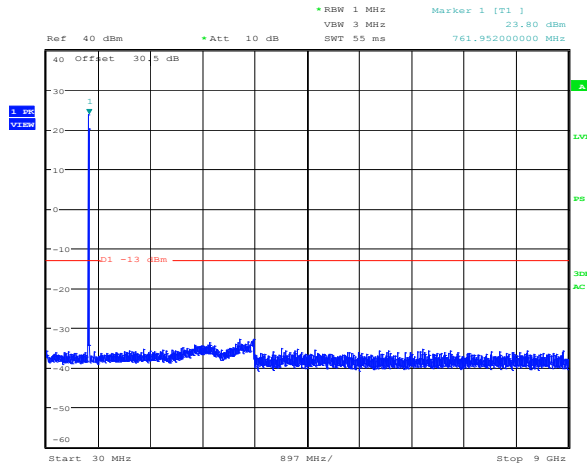
Plot 8.4-6: Spurious emissions Regular + power amplifier Downlink 700 MHz OpenSky modulation 763.00625 MHz
