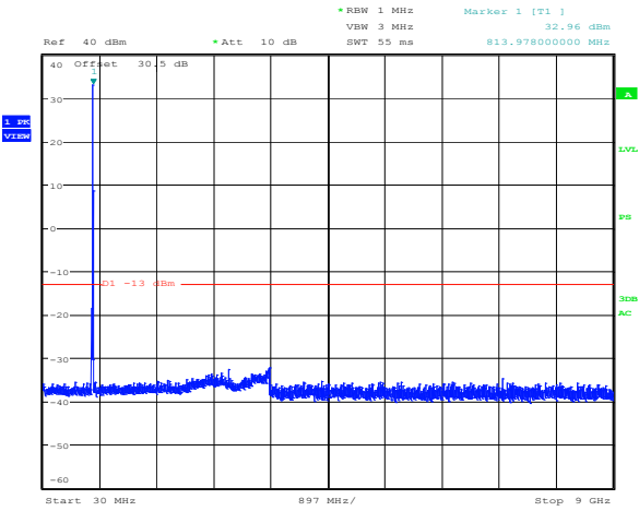
Plot 8.4-37: Spurious emissions Regular + power amplifier Uplink 800 MHz LSM modulation 815 MHz
