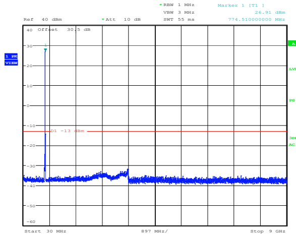
Plot 8.4-14: Spurious emissions Regular + power amplifier Downlink 700 MHz OpenSky modulation 774.99375 MHz
