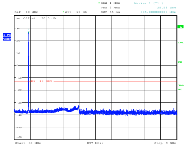
Plot 8.4-26: Spurious emissions Regular + power amplifier Uplink 800 MHz CQPSK modulation 806.00625 MHz
