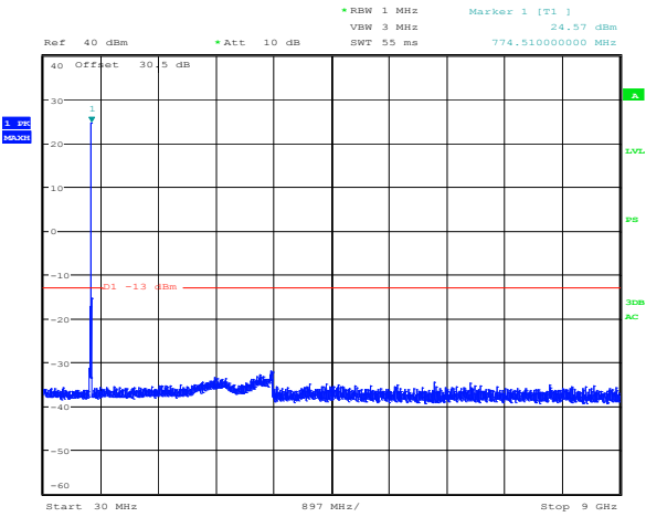
Plot 8.4-13: Spurious emissions Regular + power amplifier Downlink 700 MHz LSM modulation 774.99375 MHz
