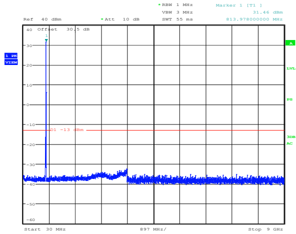
Plot 8.4-38: Spurious emissions Regular + power amplifier Uplink 800 MHz OpenSky modulation 815 MHz
