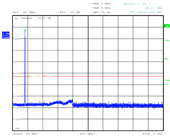
Plot 8.4-1: Spurious emissions Regular + power amplifier Downlink 700 MHz C4FM modulation 763.00625 MHz
