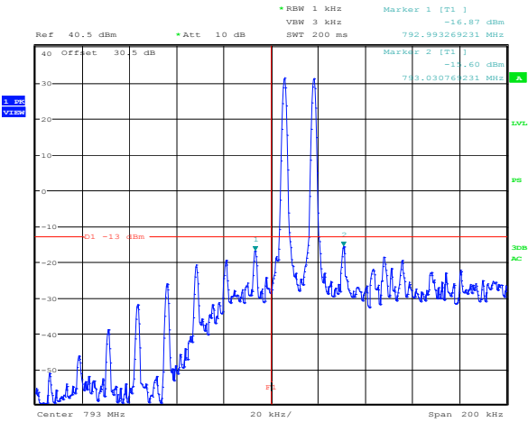
Plot 8.4-117: 3 rd order intermodulation Regular + power amplifier Uplink 700 MHz Lower band edge
