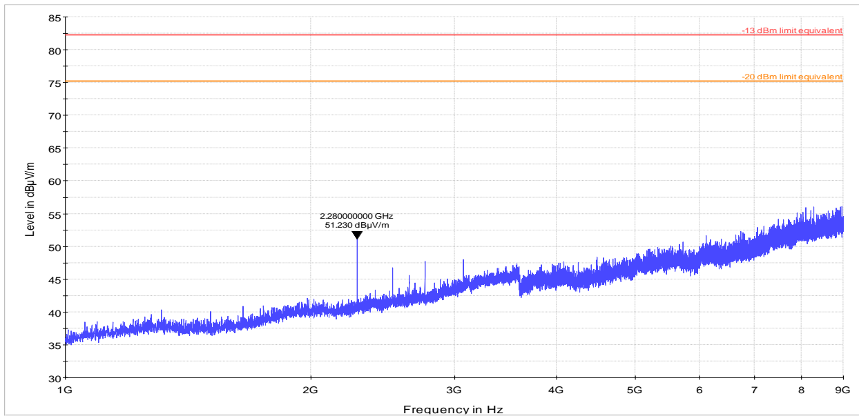
Plot 8.4-74: Radiated spurious emissions Regular + power amplifier Downlink 700 MHz
