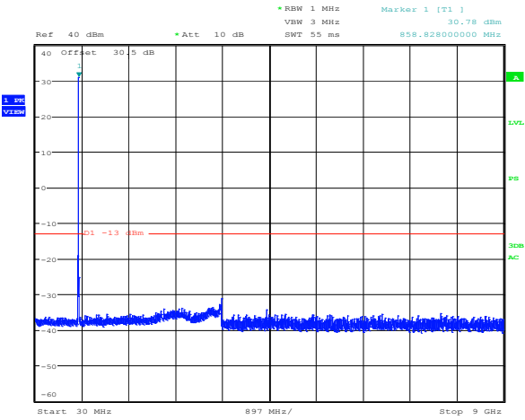
Plot 8.4-61: Spurious emissions Regular + power amplifier Downlink 800 MHz LSM modulation 860 MHz
