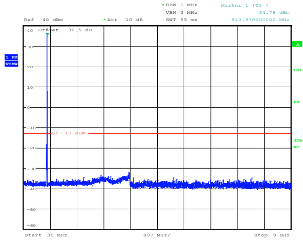
Plot 8.4-34: Spurious emissions Regular + power amplifier Uplink 800 MHz CQPSK modulation 815 MHz
