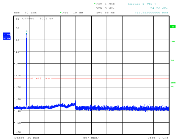
Plot 8.4-2: Spurious emissions Regular + power amplifier Downlink 700 MHz CQPSK modulation 763.00625 MHz
