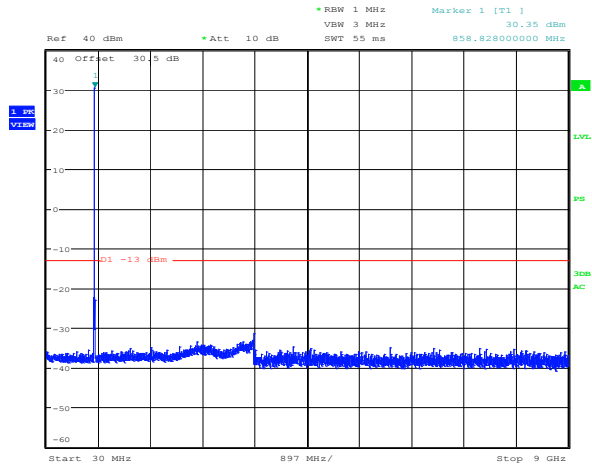
Plot 8.4-62: Spurious emissions Regular + power amplifier Downlink 800 MHz OpenSky modulation 860 MHz
