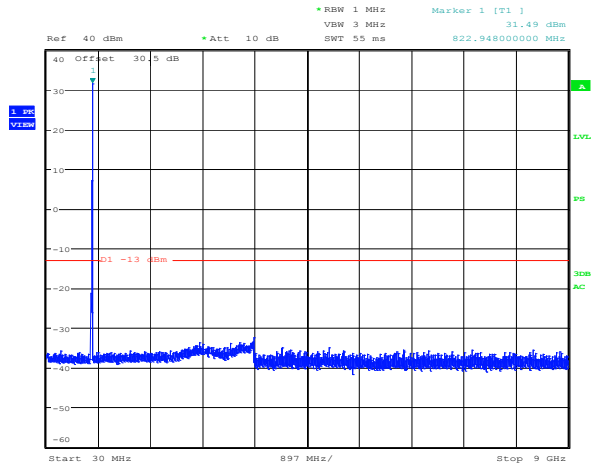
Plot 8.4-46: Spurious emissions Regular + power amplifier Uplink 800 MHz OpenSky modulation 823.99375 MHz
