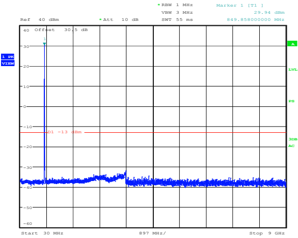
Plot 8.4-49: Spurious emissions Regular + power amplifier Downlink 800 MHz C4FM modulation 851.00625 MHz
