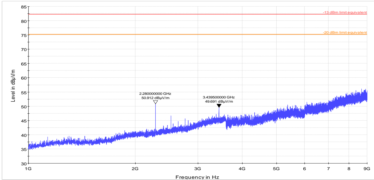
Plot 8.4-76: Radiated spurious emissions Regular + power amplifier Downlink 800 MHz
