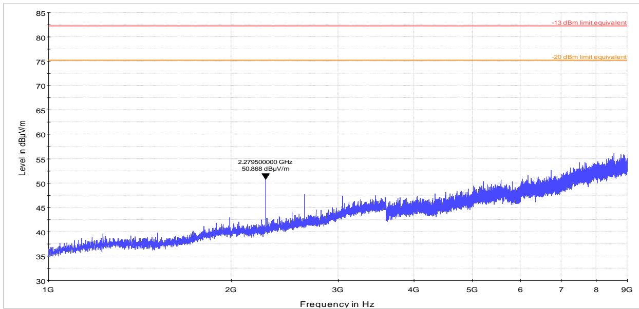
Plot 8.4-82: Radiated spurious emissions Regular high power Downlink 700 MHz
