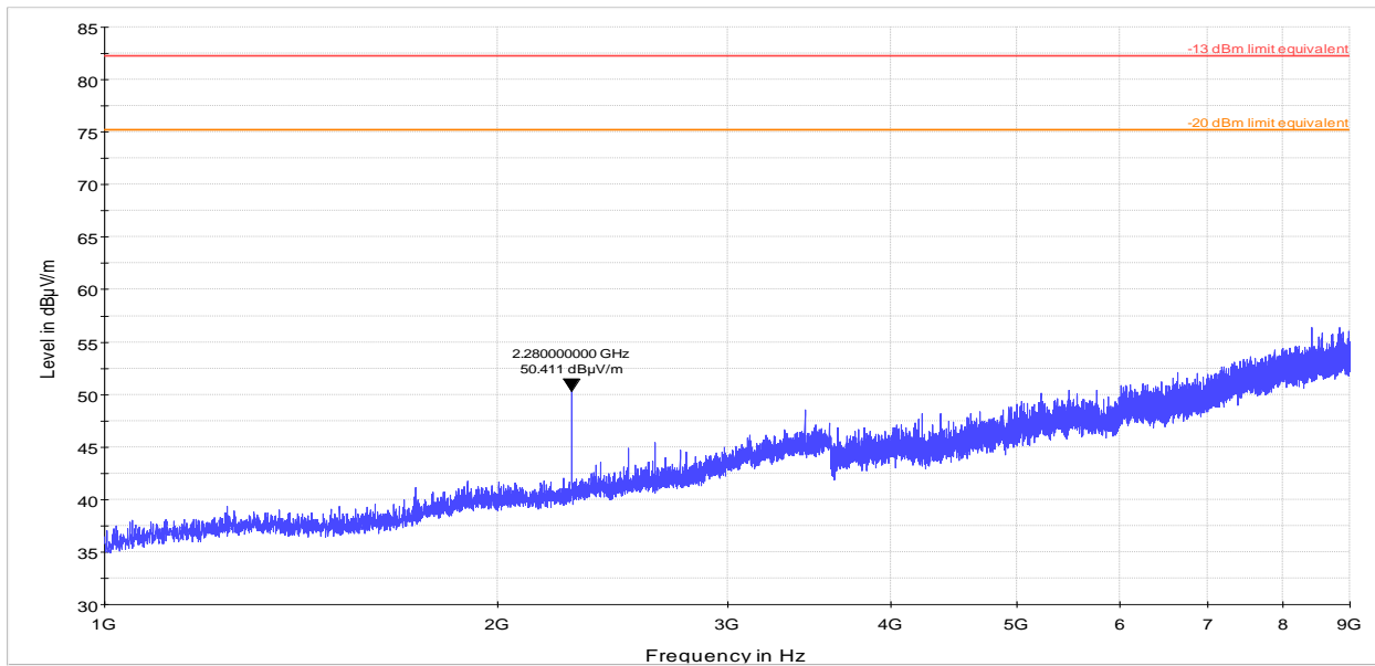
Plot 8.4-84: Radiated spurious emissions Regular high power Downlink 800 MHz
