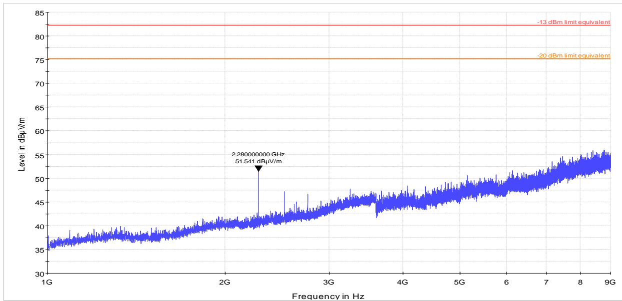
Plot 8.4-80: Radiated spurious emissions Regular + power amplifier Uplink 800 MHz
