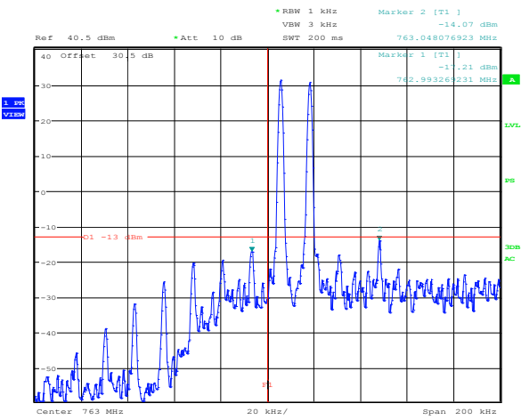
Plot 8.4-113: 3 rd order intermodulation Regular + power amplifier Downlink 700 MHz Lower band edge
