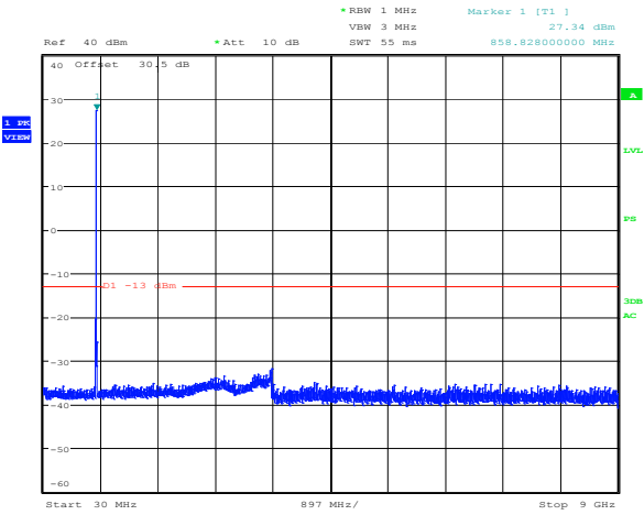
Plot 8.4-57: Spurious emissions Regular + power amplifier Downlink 800 MHz C4FM modulation 860 MHz
