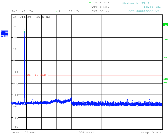
Plot 8.4-29: Spurious emissions Regular + power amplifier Uplink 800 MHz LSM modulation 806.00625 MHz
