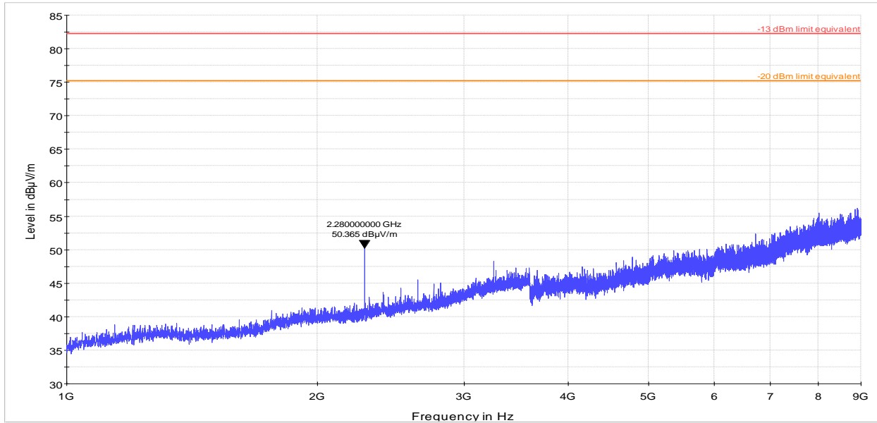
Plot 8.4-88: Radiated spurious emissions Regular high power Uplink 800 MHz
