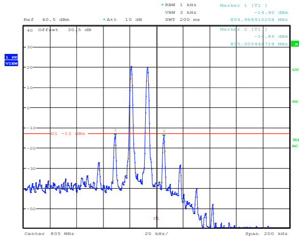
Plot 8.4-110: 3 rd order intermodulation Regular high power Uplink 700 MHz Upper band edge
