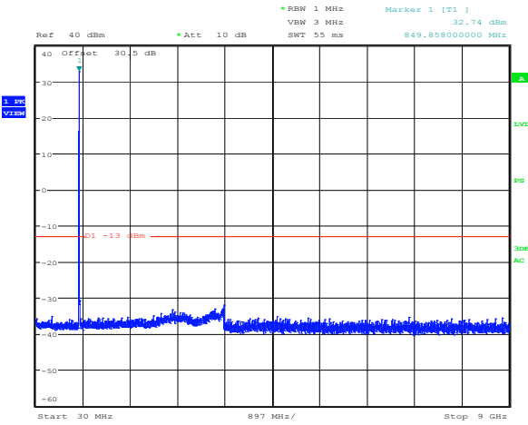
Plot 8.4-53: Spurious emissions Regular + power amplifier Downlink 800 MHz LSM modulation 851.00625 MHz
