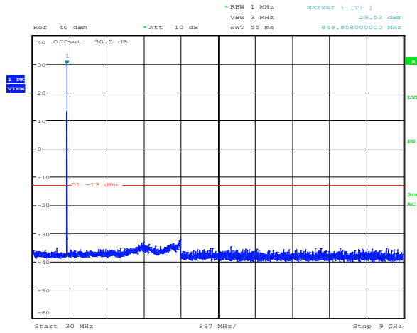
Plot 8.4-50: Spurious emissions Regular + power amplifier Downlink 800 MHz CQPSK modulation 851.00625 MHz
