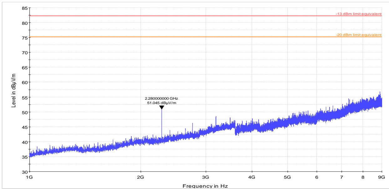
Plot 8.4-86: Radiated spurious emissions Regular high power Uplink 700 MHz
