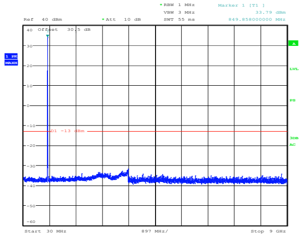
Plot 8.4-54: Spurious emissions Regular + power amplifier Downlink 800 MHz OpenSky modulation 851.00625 MHz
