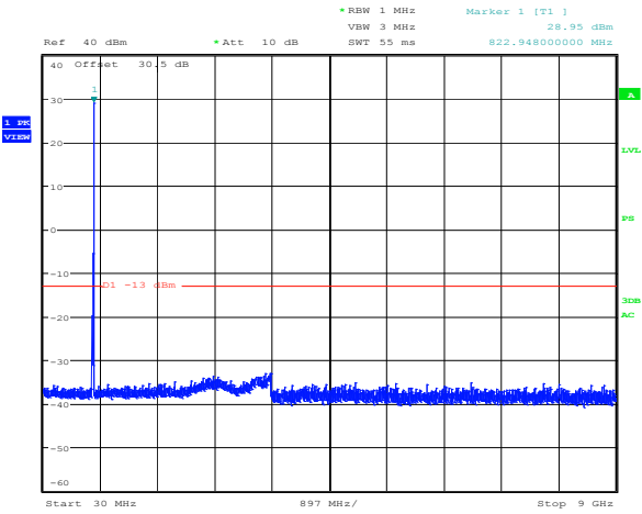
Plot 8.4-41: Spurious emissions Regular + power amplifier Uplink 800 MHz C4FM modulation 823.99375 MHz
