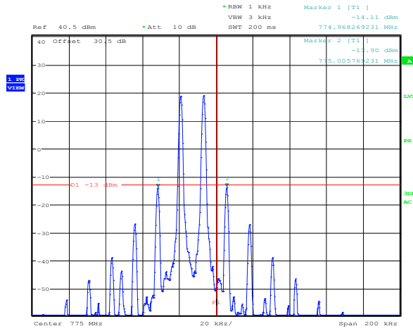
Plot 8.4-90: 3 rd order intermodulation Fiber optic high power Downlink 700 MHz Upper band edge
