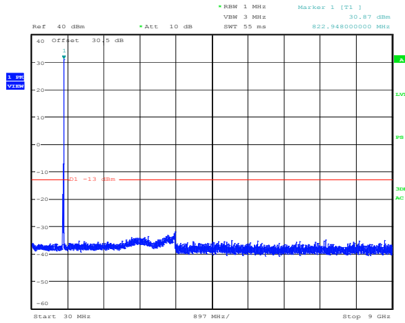
Plot 8.4-42: Spurious emissions Regular + power amplifier Uplink 800 MHz CQPSK modulation 823.99375 MHz
