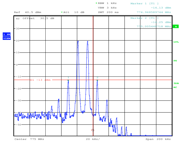
Plot 8.4-106: 3 rd order intermodulation Regular high power Downlink 700 MHz Upper band edge
