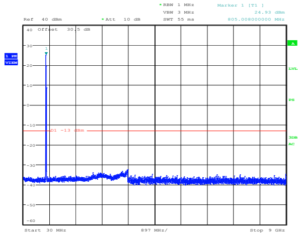
Plot 8.4-30: Spurious emissions Regular + power amplifier Uplink 800 MHz OpenSky modulation 806.00625 MHz
