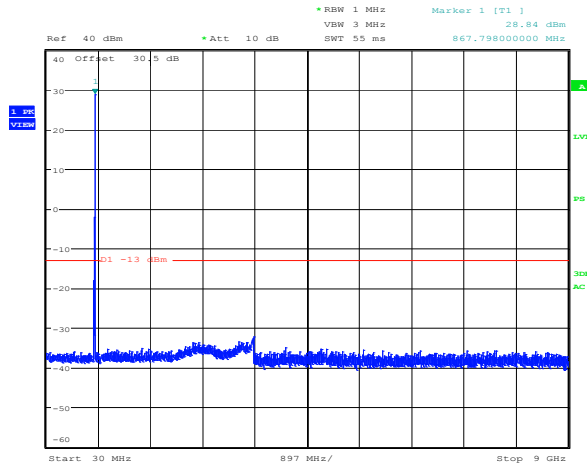
Plot 8.4-66: Spurious emissions Regular + power amplifier Downlink 800 MHz CQPSK modulation 868.99375 MHz
