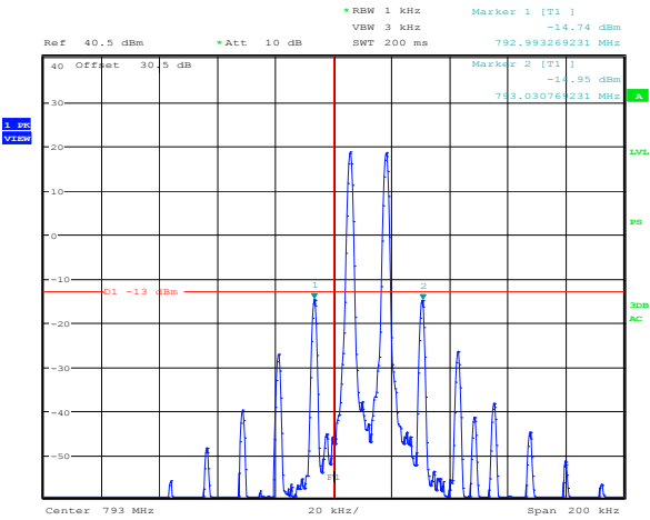
Plot 8.4-93: 3 rd order intermodulation Fiber optic high power Uplink 700 MHz Lower band edge
