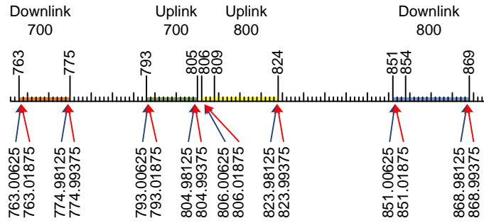
Diagram 8.4-2: Intermodulation channels
