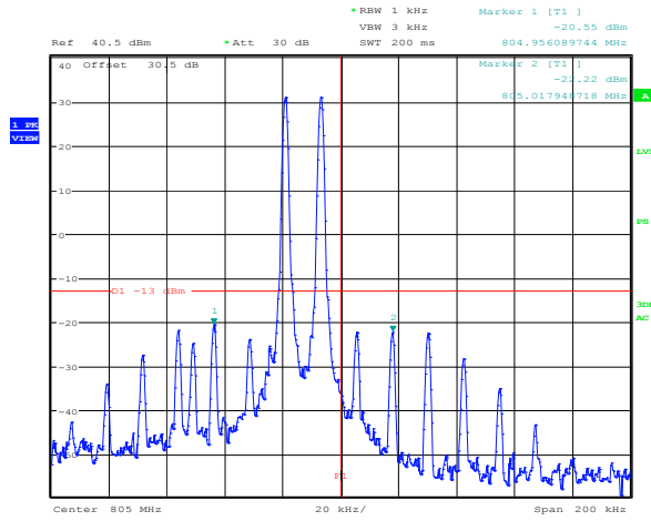
Plot 8.4-102: 3 rd order intermodulation Fiber optic + power amplifier Uplink 700 MHz Upper band edge
