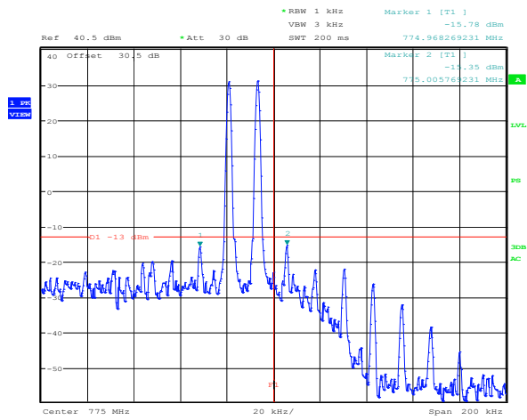
Plot 8.4-114: 3 rd order intermodulation Regular + power amplifier Downlink 700 MHz Upper band edge
