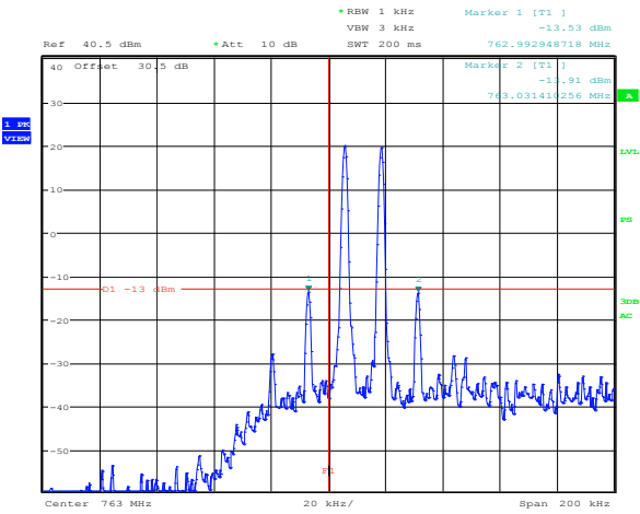
Plot 8.4-105: 3 rd order intermodulation Regular high power Downlink 700 MHz Lower band edge
