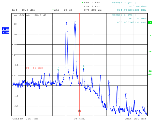
Plot 8.4-118: 3 rd order intermodulation Regular + power amplifier Uplink 700 MHz Upper band edge
