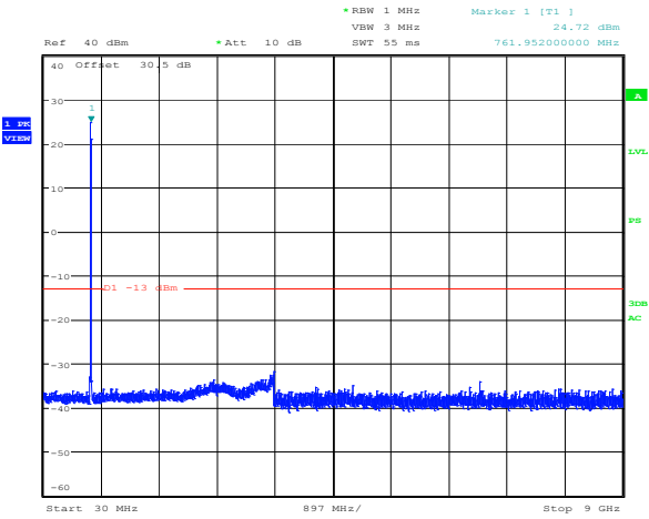
Plot 8.4-5: Spurious emissions Regular + power amplifier Downlink 700 MHz LSM modulation 763.00625 MHz
