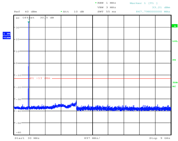
Plot 8.4-70: Spurious emissions Regular + power amplifier Downlink 800 MHz OpenSky modulation 868.99375 MHz
