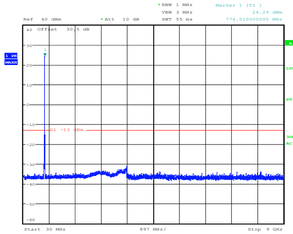
Plot 8.4-10: Spurious emissions Regular + power amplifier Downlink 700 MHz CQPSK modulation 774.99375 MHz
