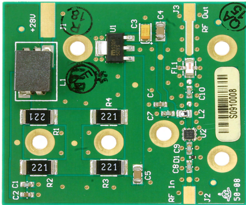
UHF Distribution Amplifier 3-22340 circuit board (3-22341) top view.
