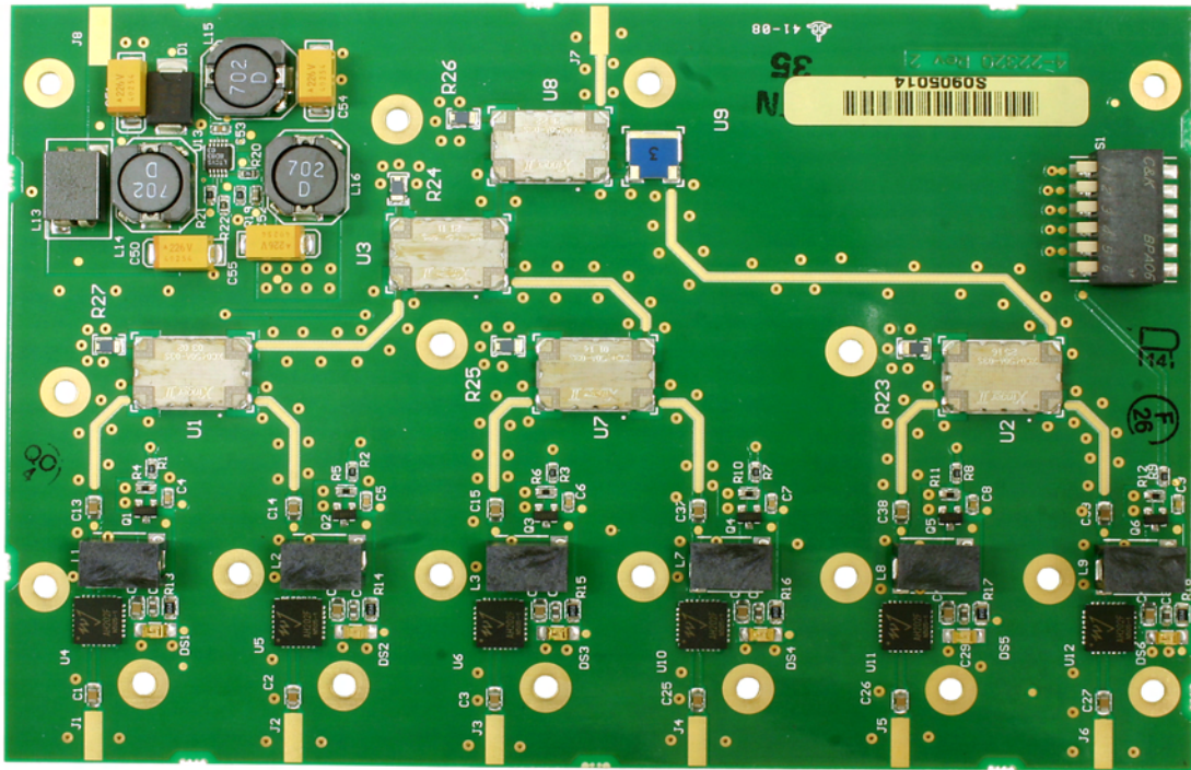
Active Combiner 3-22318 circuit board (3-22319) top view.
