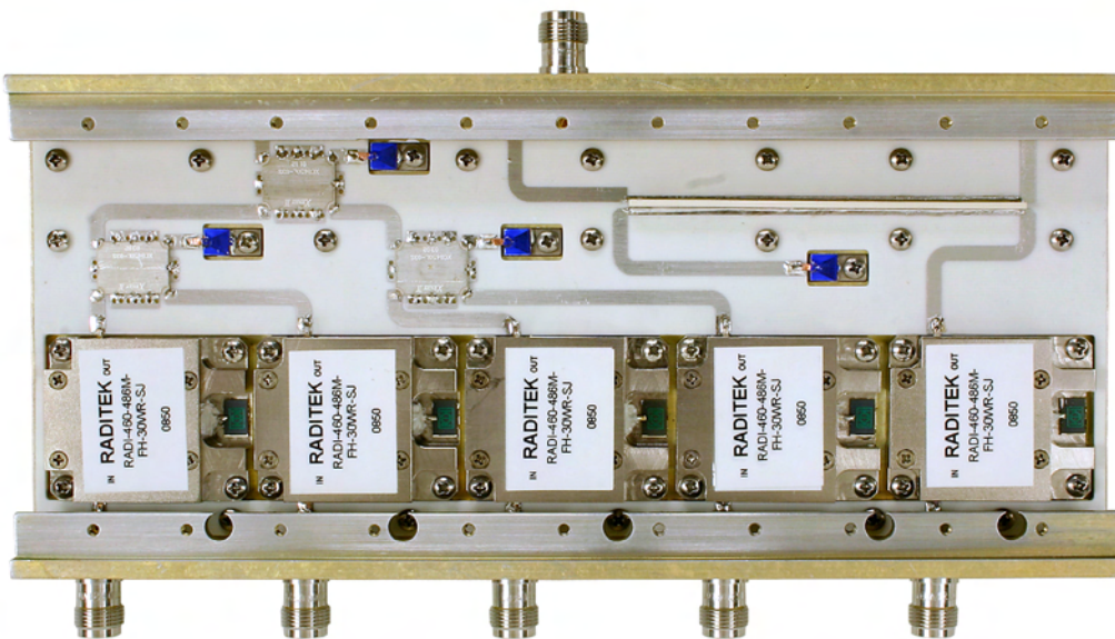
Hybrid Combiner 3-18317-1 with Circuit Board installed in chassis.
