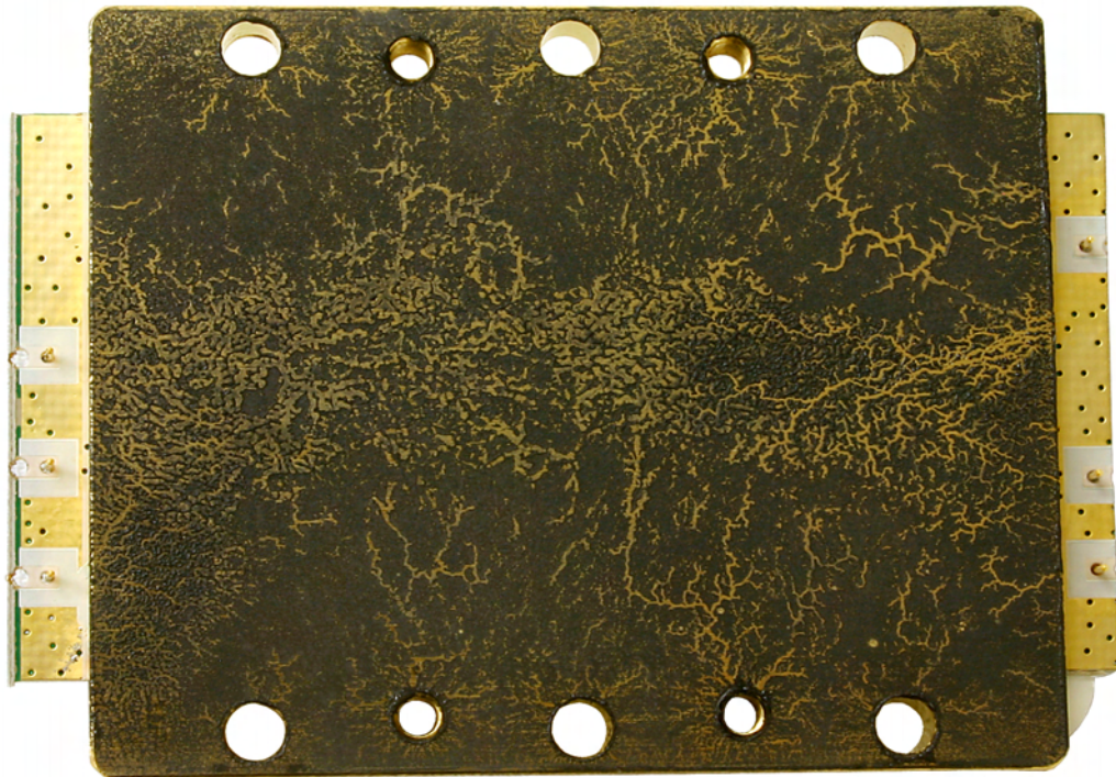
Power Amplifier 8-23291 non-component side view.
