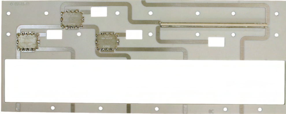
Hybrid Combiner 3-18317-1 Circuit Board top view.
