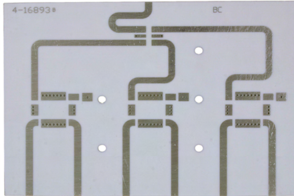
6-Way Power Divider 3-16676 Circuit Board top view.
