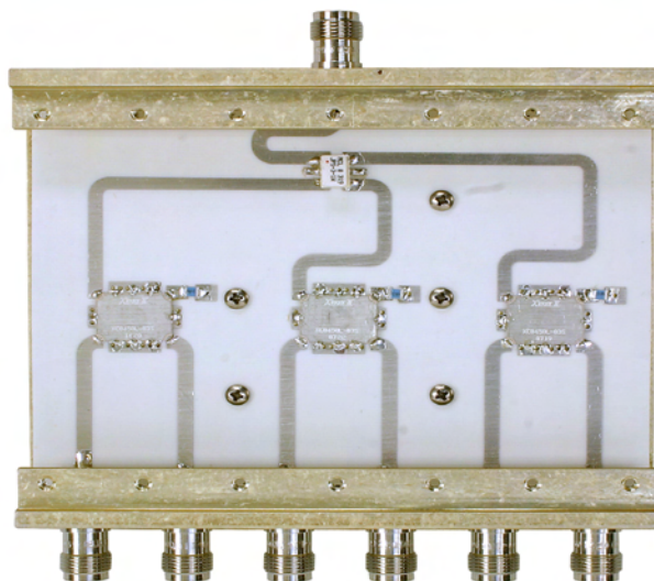
6-Way Power Divider 3-16676 with circuit board installed in chassis.
