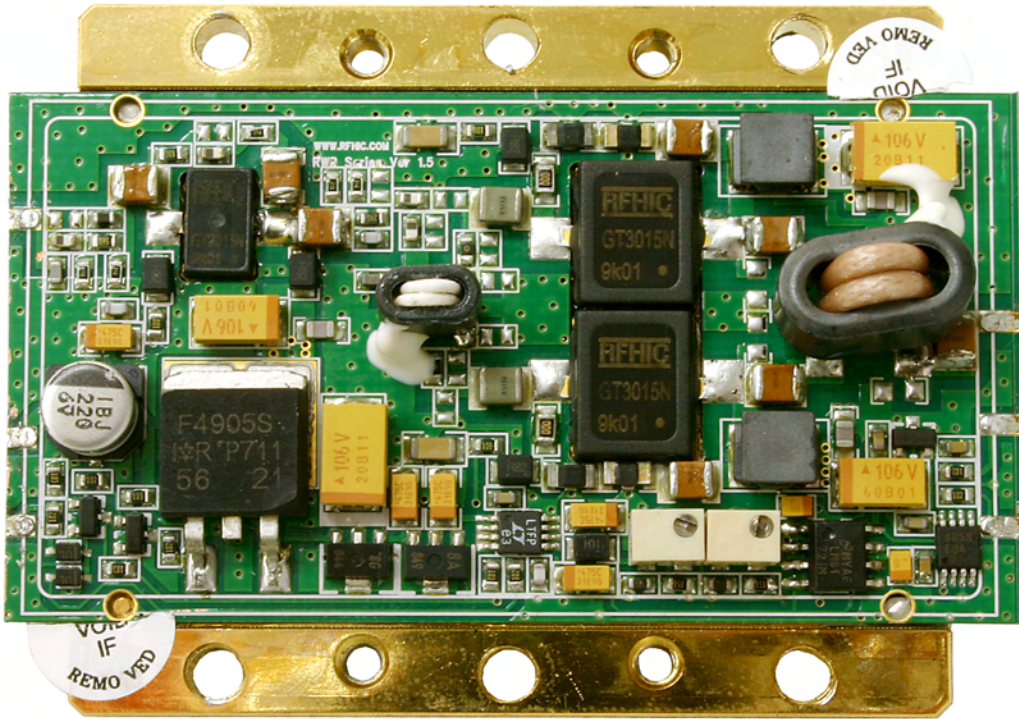
Power Amplifier 8-23291 component side view.
