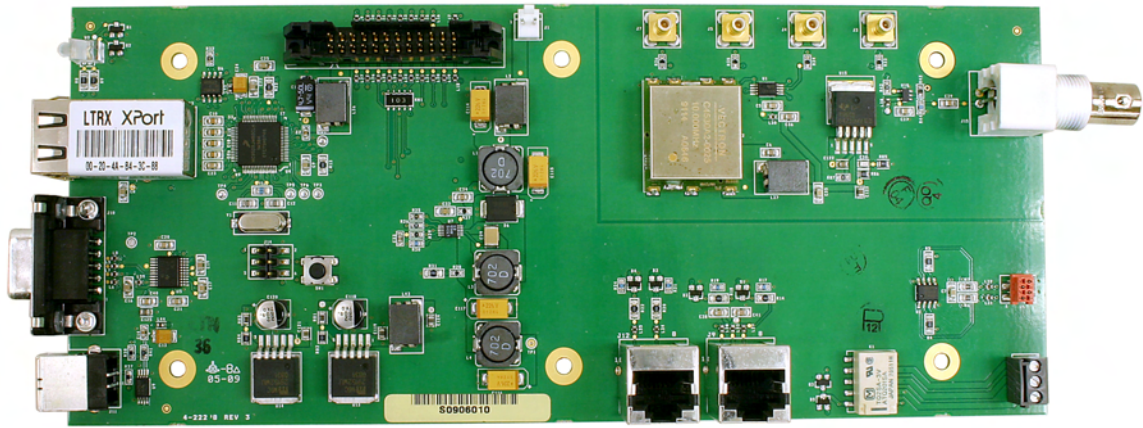
Control Board for Channel Modules 3-22297 top view.
