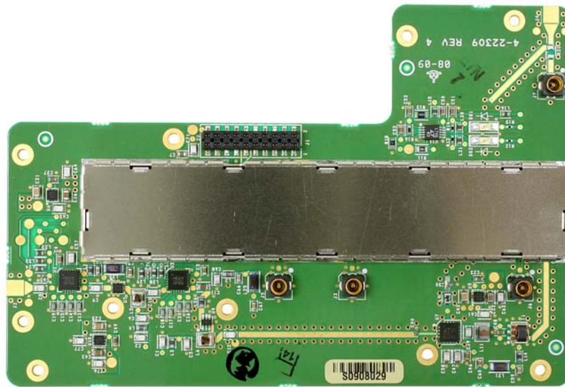
Channel Module - Down Converter Board 3-22308 top view.
