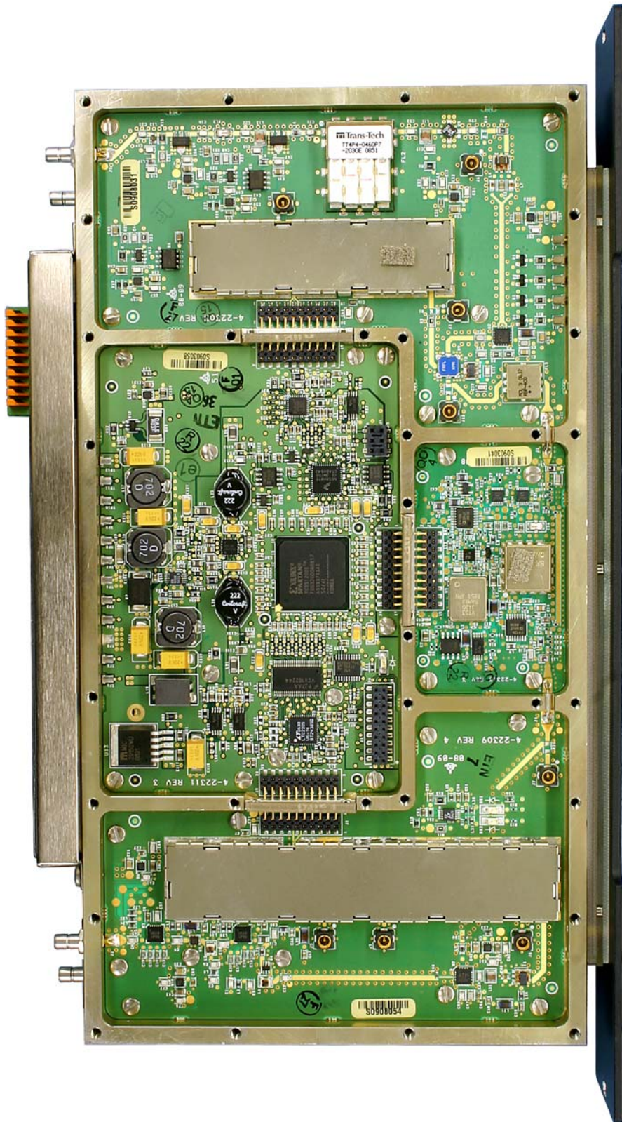
Channel Module 3-2322 with boards installed and cover removed.
