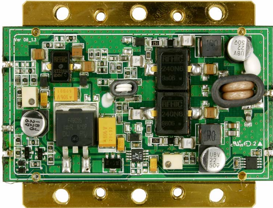
Power Amplifier 8-22290 component side view.
