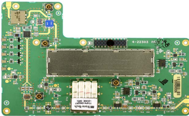
Channel Module - Up Converter Board 3-22302 top view.
