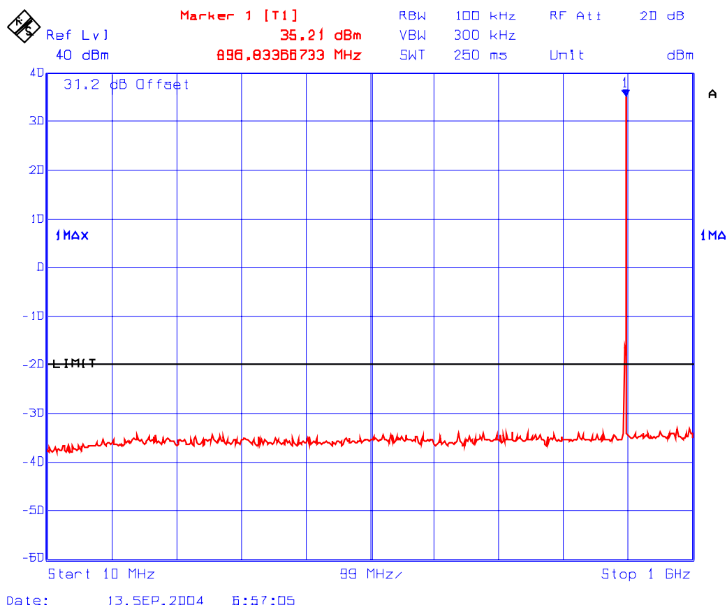
PLOT # 47 Transmitter Conducted Spurious Emissions with 1 RF signal input/output Fc: 896 MHz
