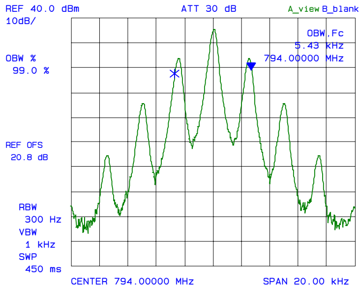
Plot 6.7.5.2.1.14: 99% Occupied Bandwidth (Output) Fc: 794 MHz, Input Level: -15 dBm, Modulation: FM with 2.5 kHz sine wave signal
