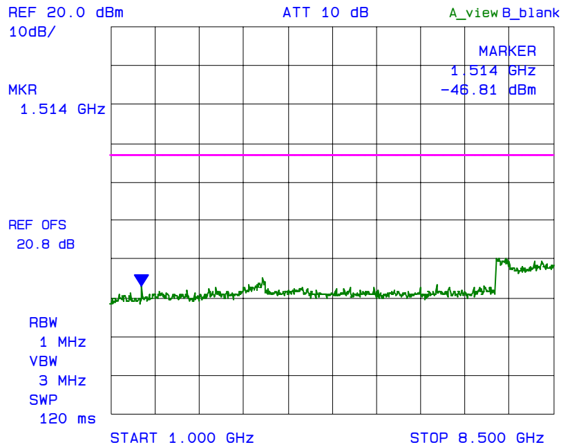
Plot 6.8.5.10 Spurious Emissions at Antenna Terminal with 2 RF signal inputs/outputs Fc: 770 MHz, Fc + 25 kHz
