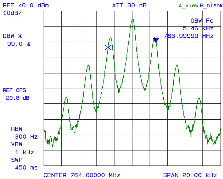
Plot 6.7.5.2.1.2: 99% Occupied Bandwidth (Output) Fc: 764 MHz, Level: -15 dBm, Modulation: FM with 2.5 kHz sine wave signal
