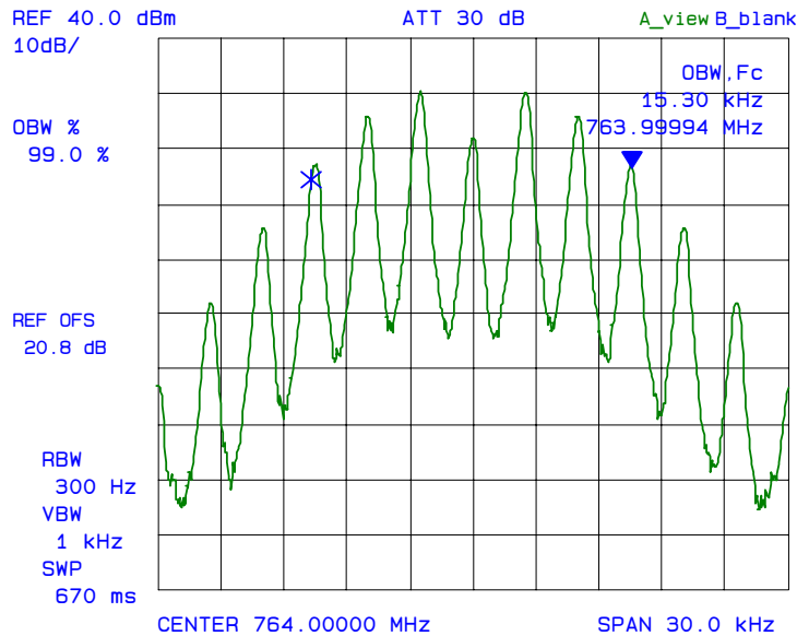
Plot 6.7.5.2.3.2: 99% Occupied Bandwidth (Output) Fc: 764 MHz, Input Level: -15 dBm, Modulation: FM with 2.5 kHz sine wave signal
