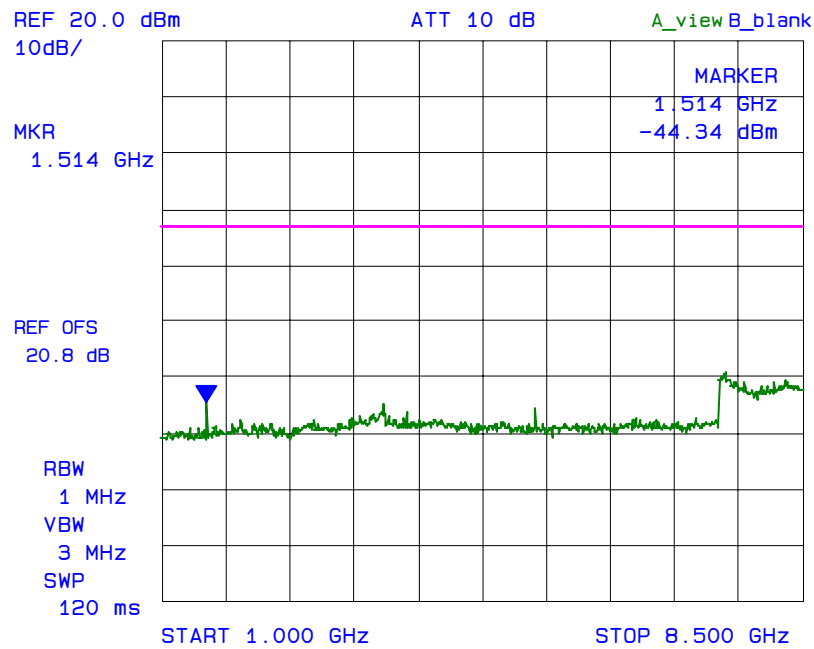
Plot 6.8.5.12 Spurious Emissions at Antenna Terminal with 3 RF signal inputs/outputs Fc: 770 MHz, Fc + 25 kHz, Fc + 50 kHz
