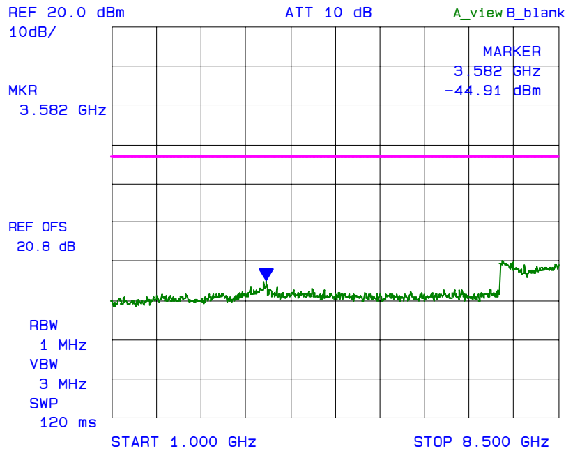
Plot 6.8.5.34 Spurious Emissions at Antenna Terminal with 2 RF signal inputs/outputs Fc: 806 MHz, Fc - 25 kHz
