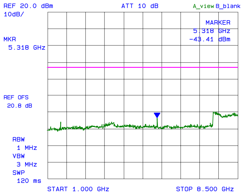
Plot 6.8.5.6 Spurious Emissions at Antenna Terminal with 3 RF signal inputs/outputs Fc: 764 MHz, Fc + 25 kHz, Fc + 50 kHz
