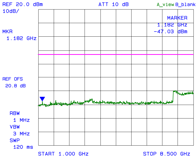
Plot 6.8.5.20 Spurious Emissions at Antenna Terminal with 1 RF signal input/output Fc: 794 MHz
