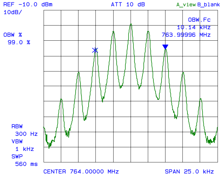
Plot 6.7.5.2.2.2: 99% Occupied Bandwidth (Output) Fc: 764 MHz, Input Level: -15 dBm, Modulation: FM with 2.5 kHz sine wave signal
