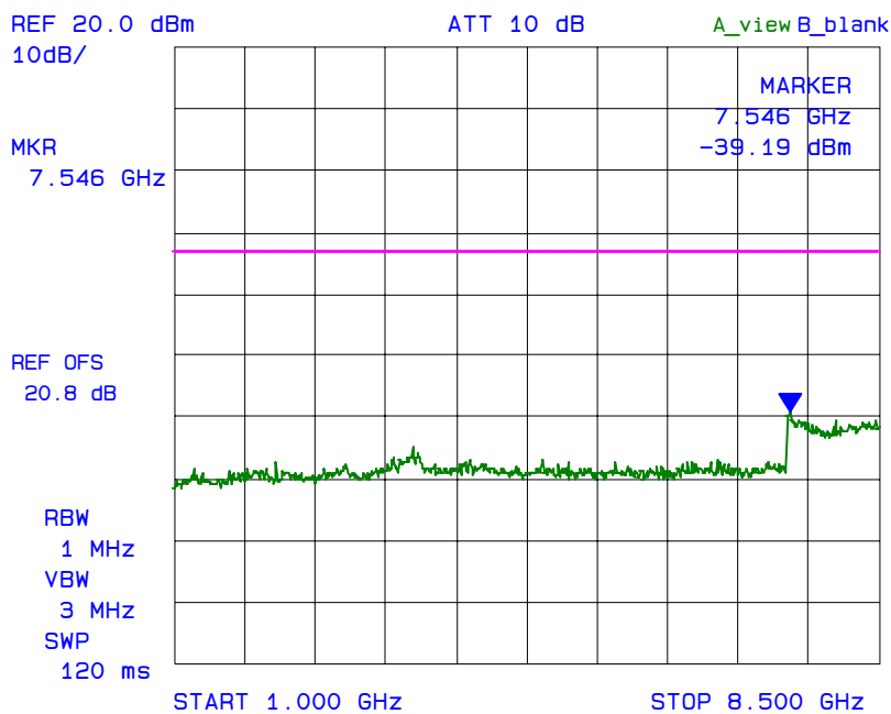
Plot 6.8.5.24 Spurious Emissions at Antenna Terminal with 3 RF signal inputs/outputs Fc: 794 MHz, Fc + 25 kHz, Fc + 50 kHz
