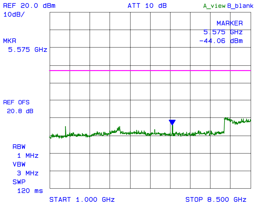
Plot 6.8.5.30 Spurious Emissions at Antenna Terminal with 3 RF signal inputs/outputs Fc: 800 MHz, Fc + 25 kHz, Fc + 50 kHz
