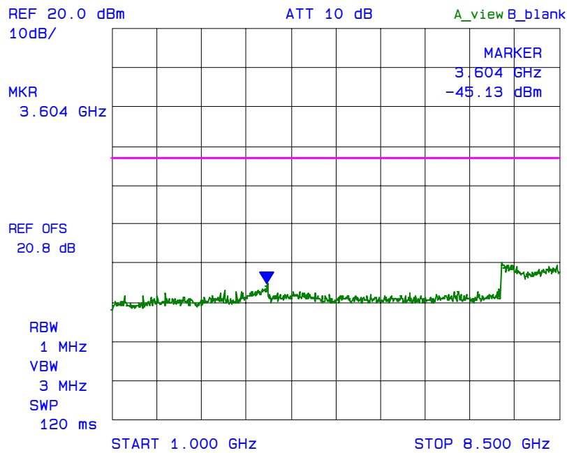
Plot 6.8.5.8 Spurious Emissions at Antenna Terminal with 1 RF signal input/output Fc: 770 MHz
