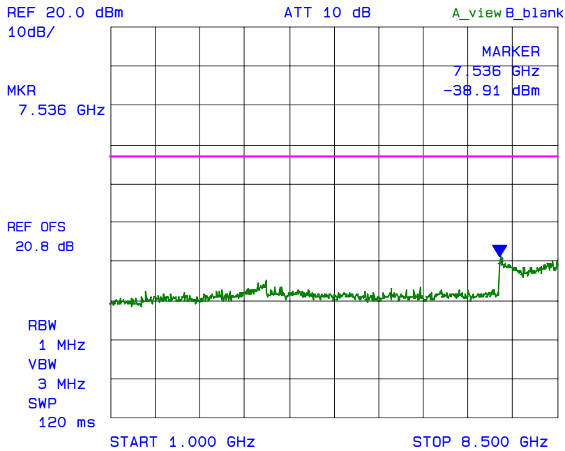
Plot 6.8.5.26 Spurious Emissions at Antenna Terminal with 1 RF signal input/output Fc: 800 MHz
