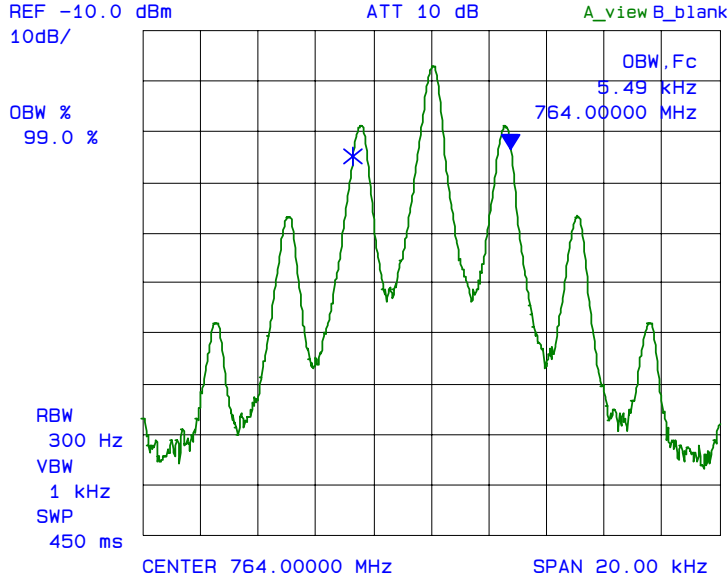
Plot 6.7.5.2.1.1: 99% Occupied Bandwidth (Input) Fc: 764 MHz, Input Level: -15 dBm, Modulation: FM with 2.5 kHz sine wave signal
