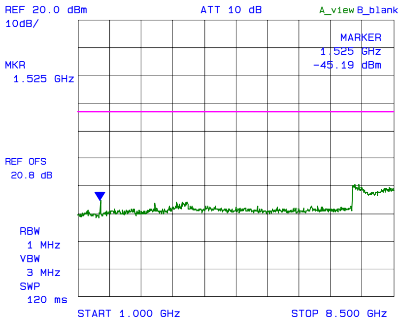
Plot 6.8.5.18 Spurious Emissions at Antenna Terminal with 3 RF signal inputs/outputs Fc: 776 MHz, Fc - 25 kHz, Fc - 50 kHz
