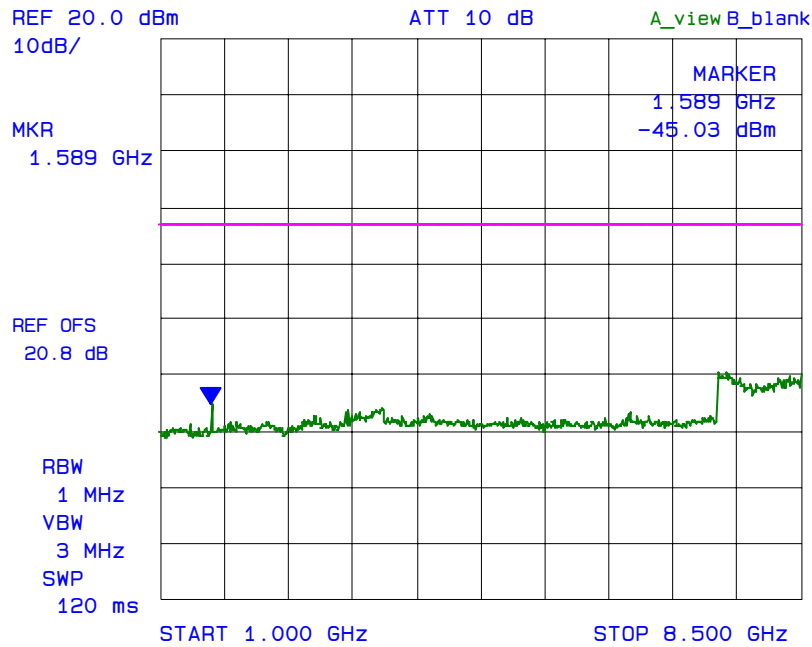
Plot 6.8.5.36 Spurious Emissions at Antenna Terminal with 3 RF signal inputs/outputs Fc: 806 MHz, Fc - 25 kHz, Fc - 50 kHz
