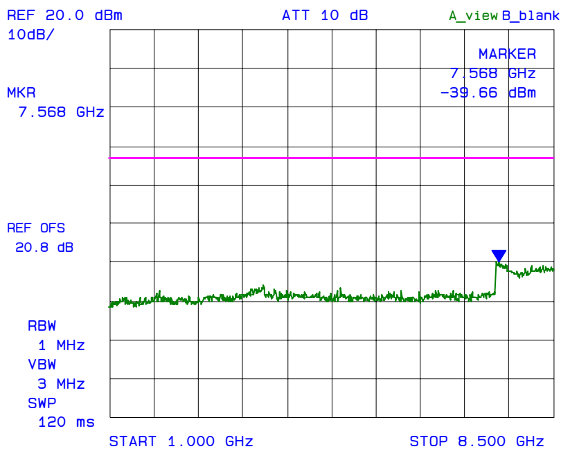
Plot 6.8.5.2 Spurious Emissions at Antenna Terminal with 1 RF signal input/output Fc: 764 MHz
