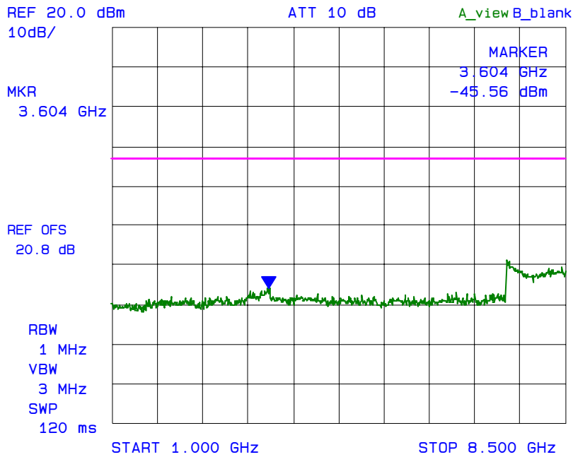
Plot 6.8.5.32 Spurious Emissions at Antenna Terminal with with 1 RF signal input/output Fc: 806 MHz
