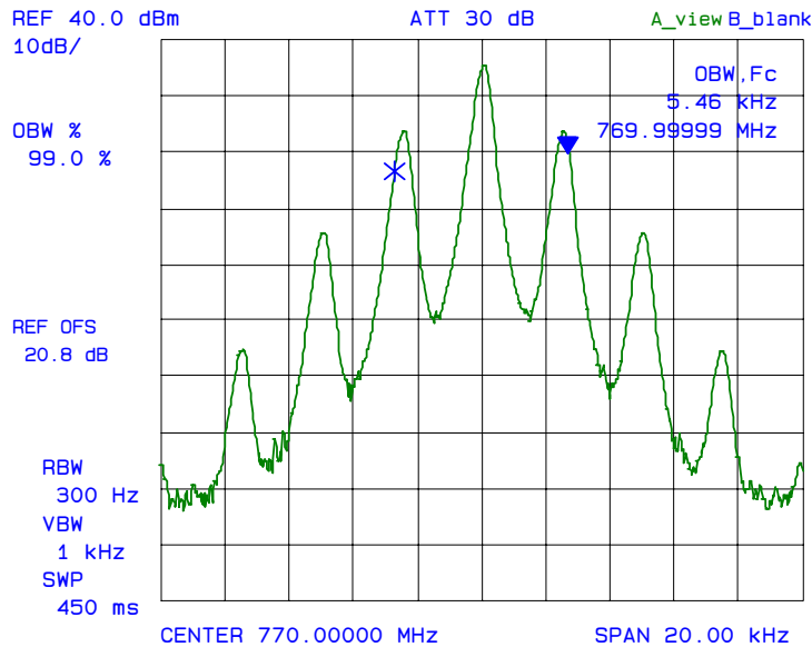
Plot 6.7.5.2.1.6: 99% Occupied Bandwidth (Output) Fc: 770 MHz, Input Level: -15 dBm, Modulation: FM with 2.5 kHz sine wave signal
