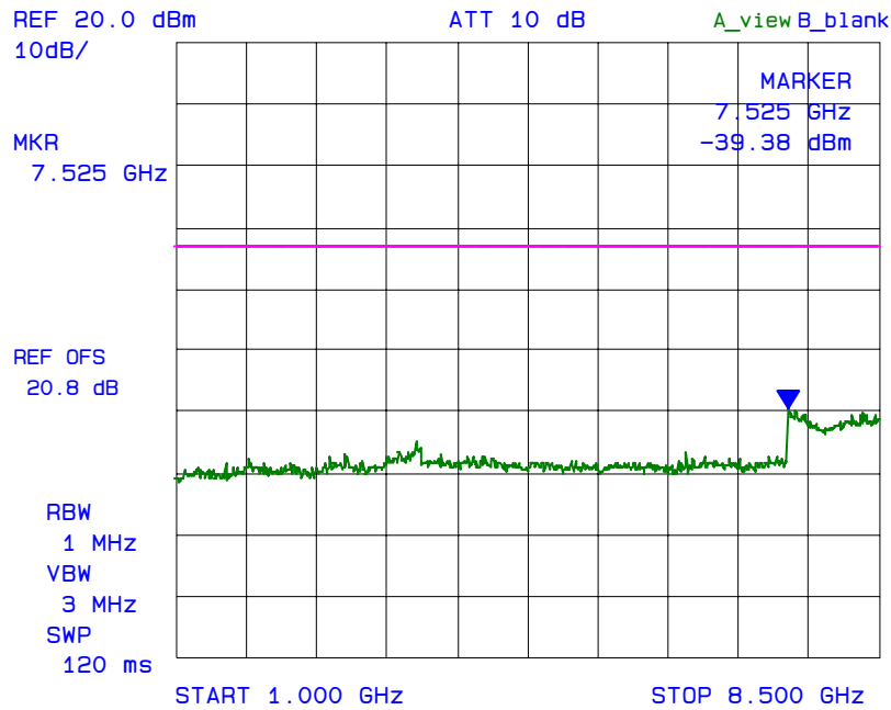
Plot 6.8.5.16 Spurious Emissions at Antenna Terminal with 2 RF signal inputs/outputs Fc: 776 MHz, Fc - 25 kHz
