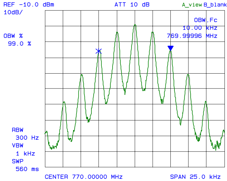
Plot 6.7.5.2.2.6: 99% Occupied Bandwidth (Output) Fc: 770 MHz, Input Level: -15 dBm, Modulation: FM with 2.5 kHz sine wave signal.
