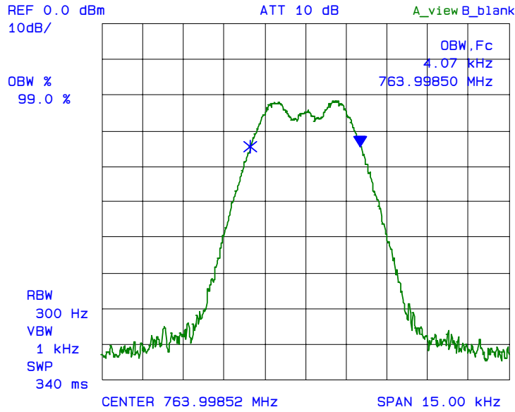
Plot 6.7.5.2.1.3: 99% Occupied Bandwidth (Input) Fc: 764 MHz, Input Level: -15 dBm, Modulation: FM with an external 9600 bps random data source
