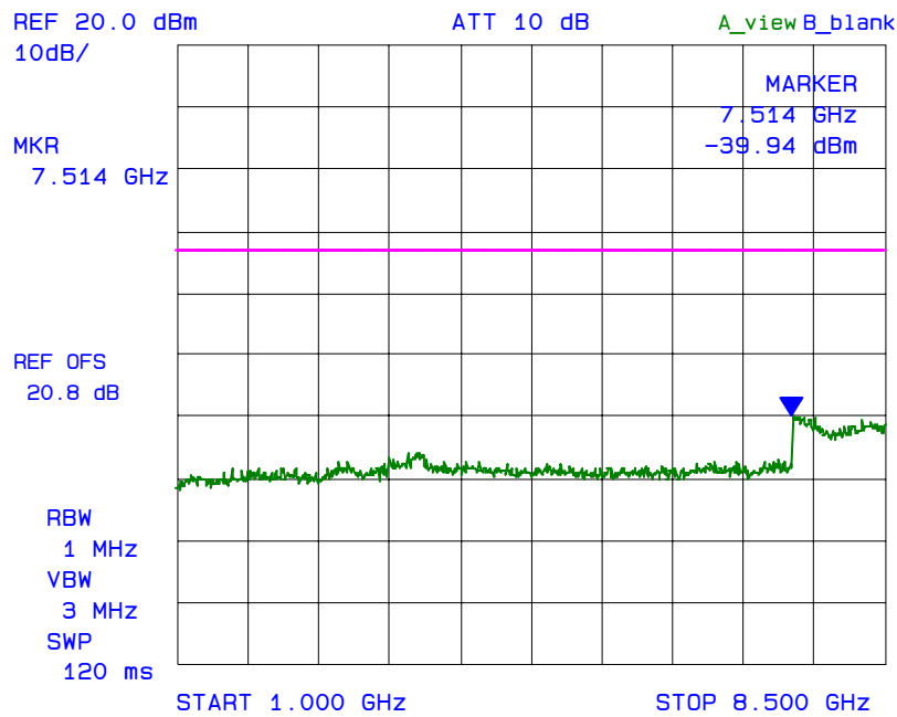
Plot 6.8.5.22 Spurious Emissions at Antenna Terminal with 2 RF signal inputs/outputs Fc: 794 MHz, Fc + 25 kHz
