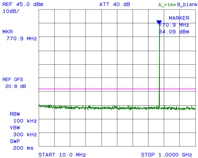
Plot 6.8.5.13 Spurious Emissions at Antenna Terminal with 1 RF signal input/output Fc: 776 MHz
