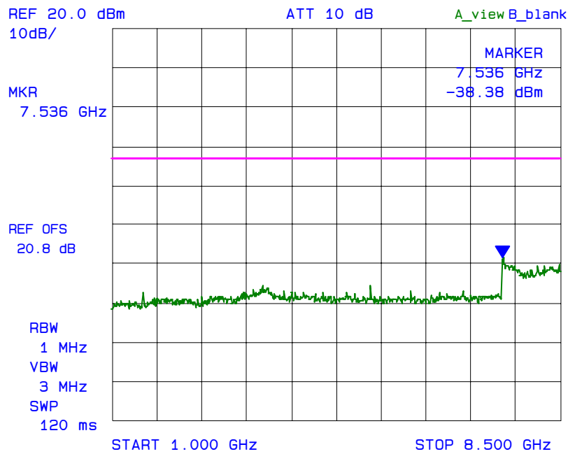
Plot 6.8.5.4 Spurious Emissions at Antenna Terminal with 2 RF signal inputs/outputs Fc: 764 MHz, Fc + 25 kHz
