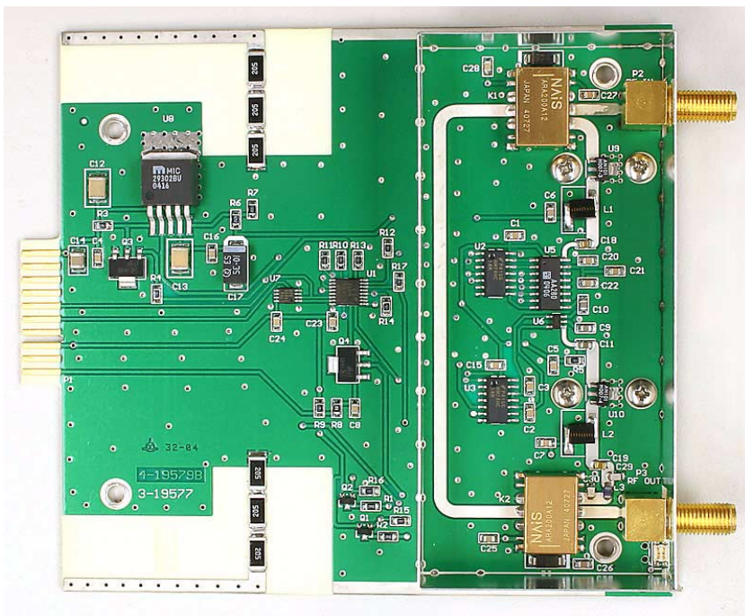
3-19576 Mid-Level Amplifier Card Front PCB View
