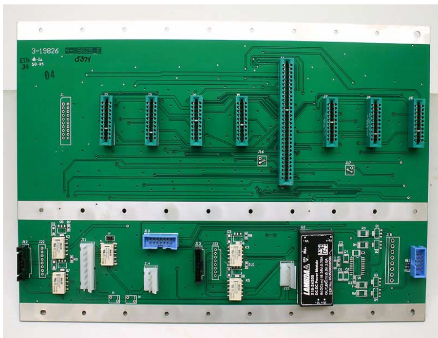
3-19826 BackPlane Circuit Board Front PCB View
