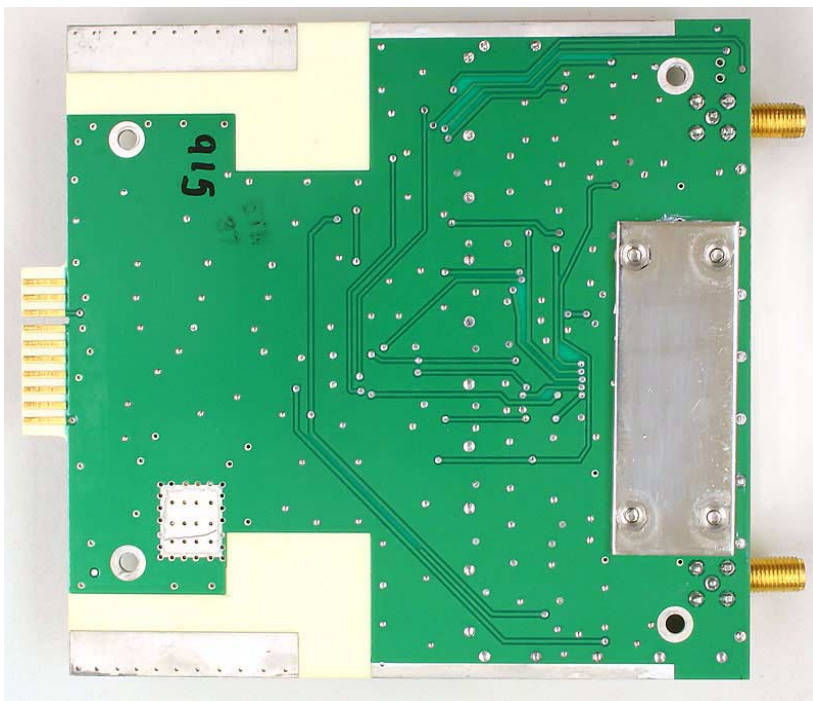
3-19576 Mid-Level Amplifier Card Back PCB View
