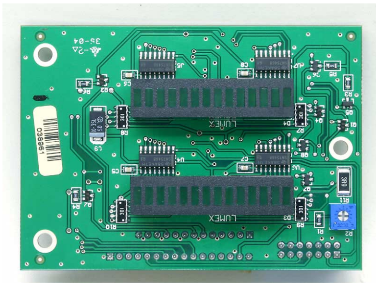
3-19708 Display Circuit Board Front PCB View
