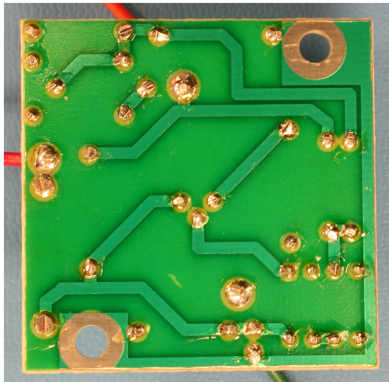
3-12809 Bias Circuit Board Assembly
