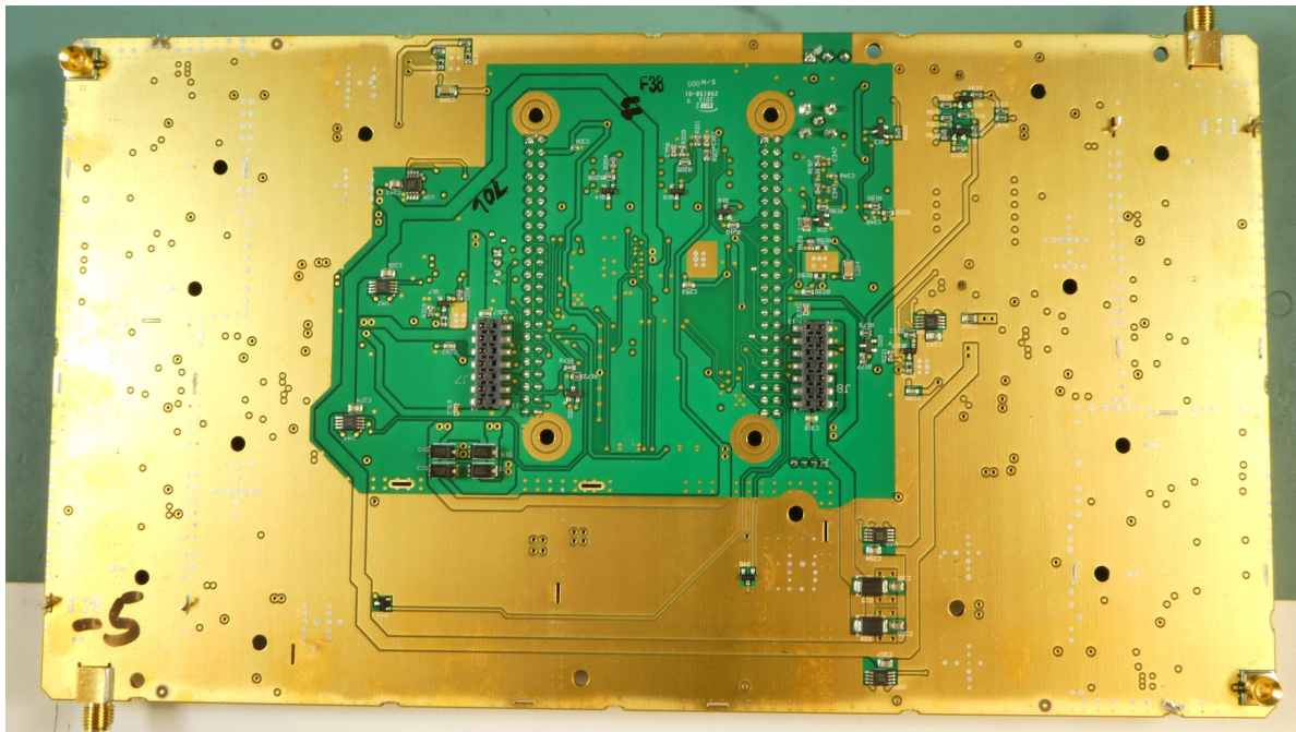
Control and LNA PCBA 3-26063-5 Rear view
