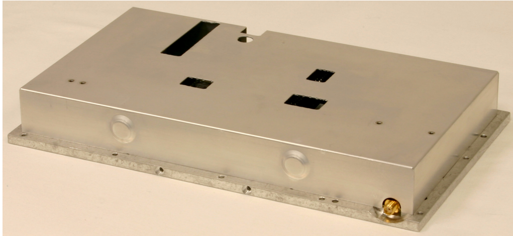
Control and LNA Assembly 3-26062-1 Rear-side view.
