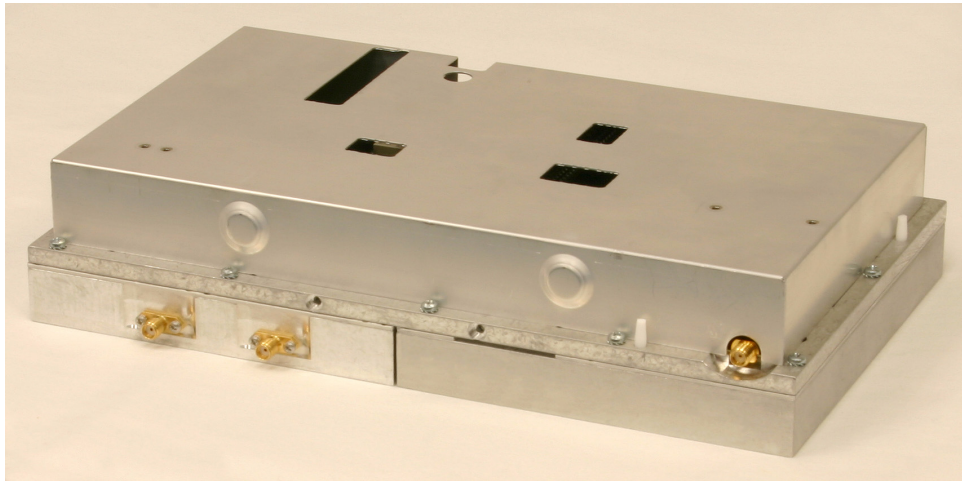
Class B SB Module 3-25999-1S, or 3-25999-2S Rear-side view.
