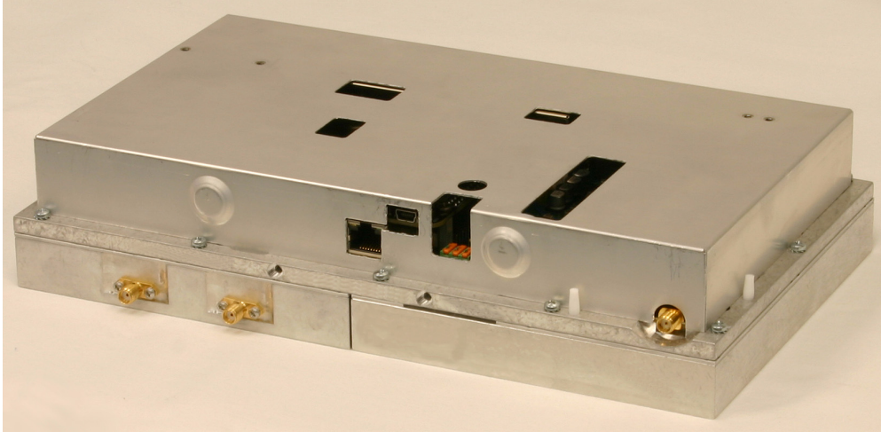
Class B SB Module 3-25999-1S, or 3-25999-2S Front-side view.
