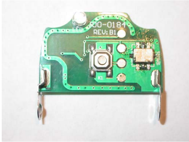
Photo 4 PCB top side
