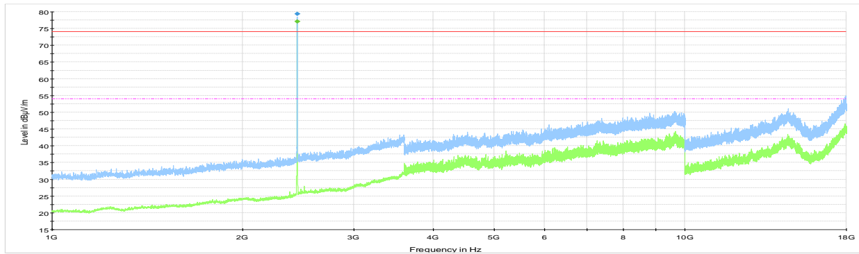
RE,1to18G, tx on mid ch Preview Result 2-AVG Preview Result 1-PK+
