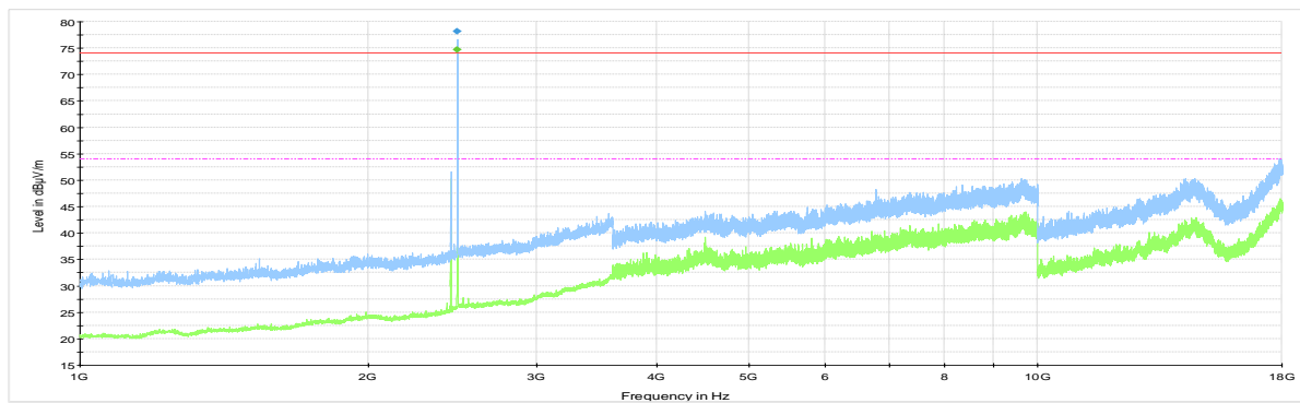
RE,1to18G, tx on high ch Preview Result 2-AVG Preview Result 1-PK+
