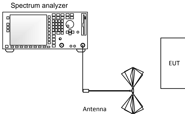
Figure 3.6-1: Setup diagram
