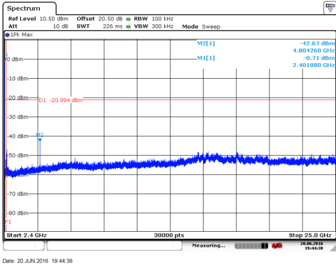
Figure 8.3-6: Conducted spurious emissions above 2.4 GHz, Low channel
