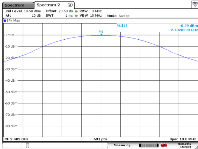
Figure 8.2-1: Low Channel
