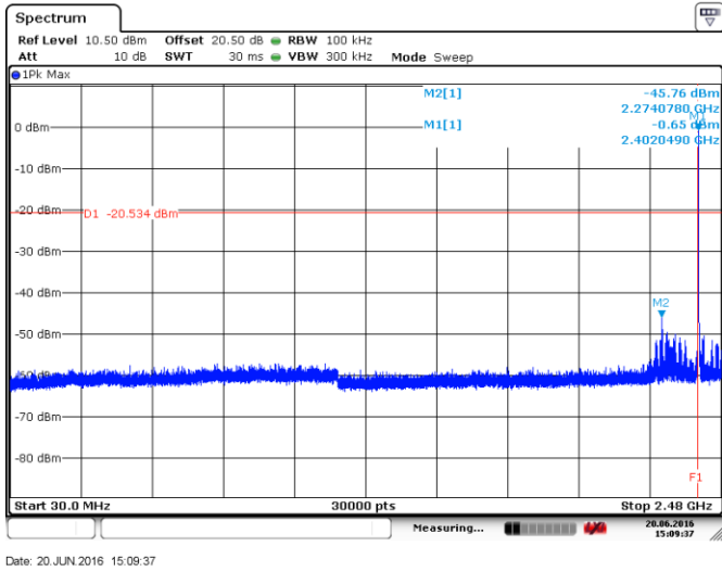
Figure 8.3-3: Conducted spurious emissions below 2.4 GHz, Low channel
