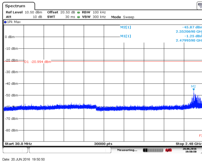
Figure 8.3-5: Conducted spurious emissions below 2.4 GHz, High channel
