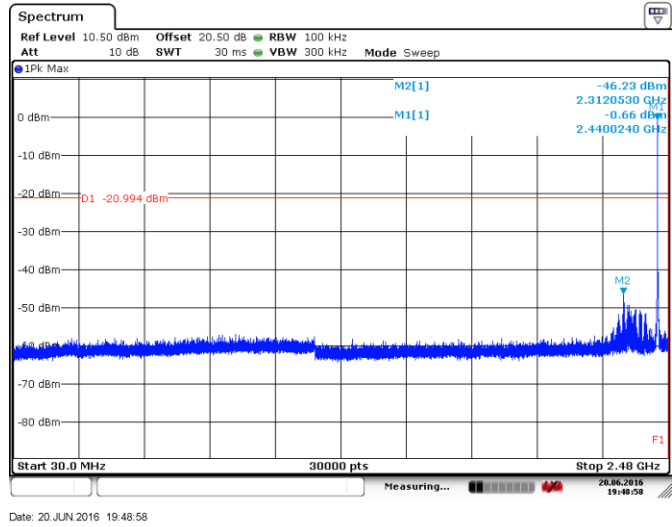
Figure 8.3-4: Conducted spurious emissions below 2.4 GHz, Mid channel
