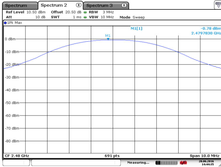
Figure 8.2-3: High Channel
