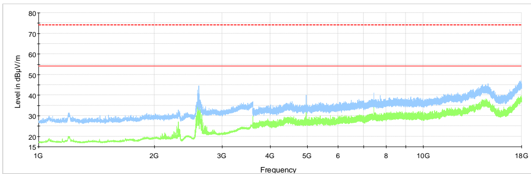
Figure 8.3-11: Radiated spurious emissions 1 to 18 GHz, High channel
