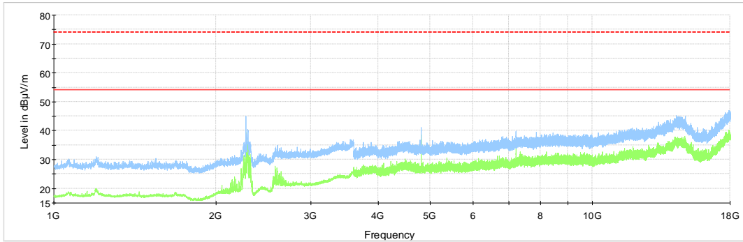
Figure 8.3-9: Radiated spurious emissions 1 to 18 GHz, Low channel
