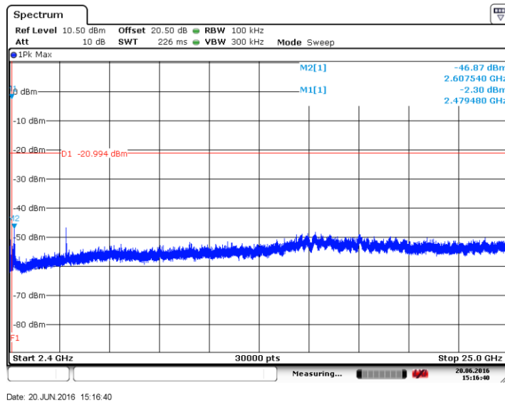
Figure 8.3-8: Conducted spurious emissions above 2.4 GHz, High channel
