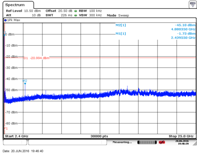
Figure 8.3-7: Conducted spurious emissions above 2.4 GHz, Mid channel
