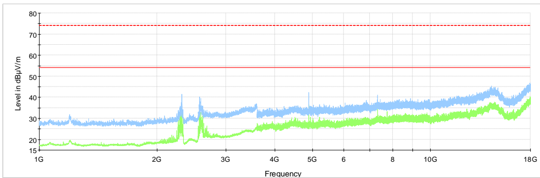
Figure 8.3-10: Radiated spurious emissions 1 to 18 GHz, Mid channel
