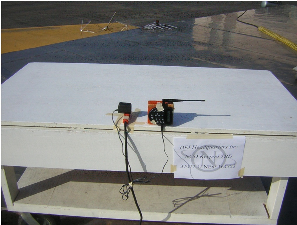
MODEL 6703A (HUB), keypad required for changing frequencies, test mode. radiated emissions
