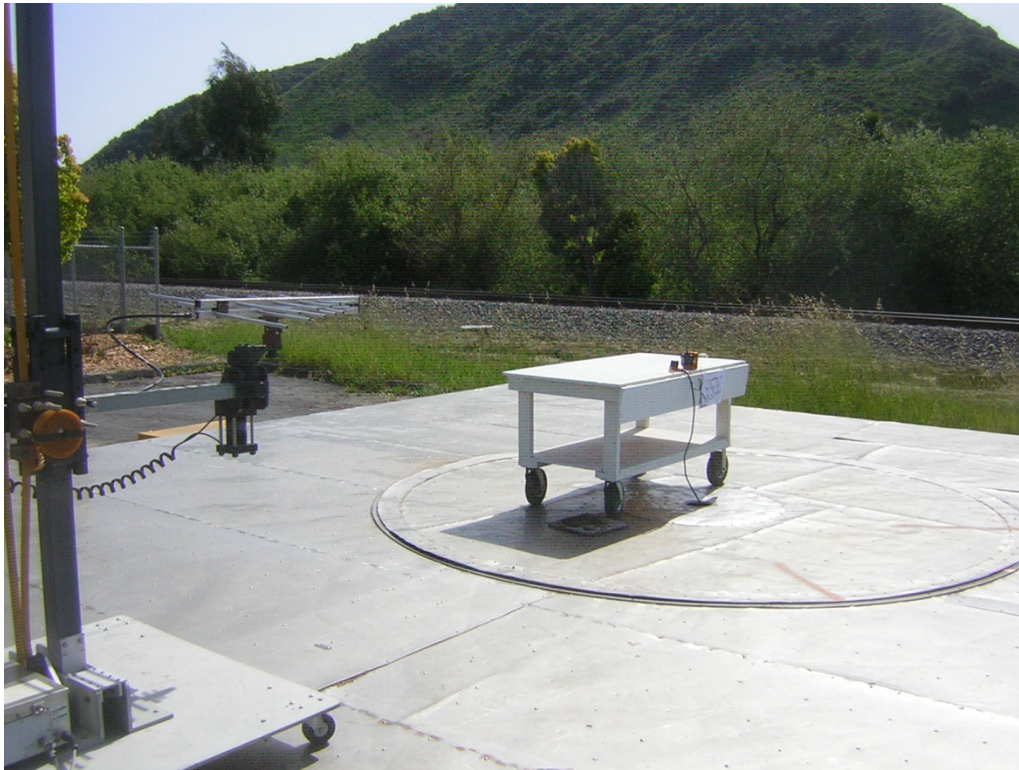
MODEL 7703A (remote) radiated emissions
