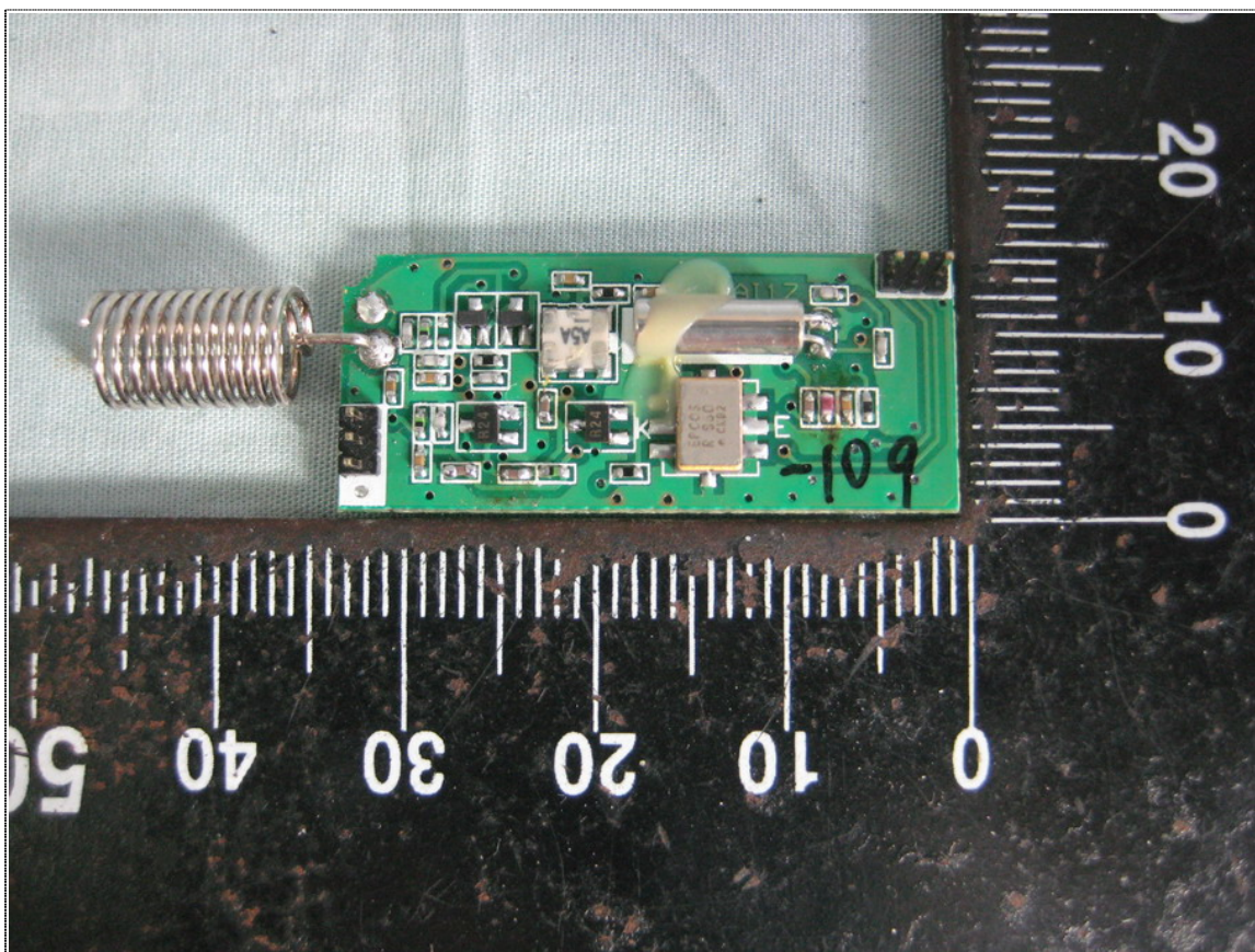
Component View of PCB Board-2
