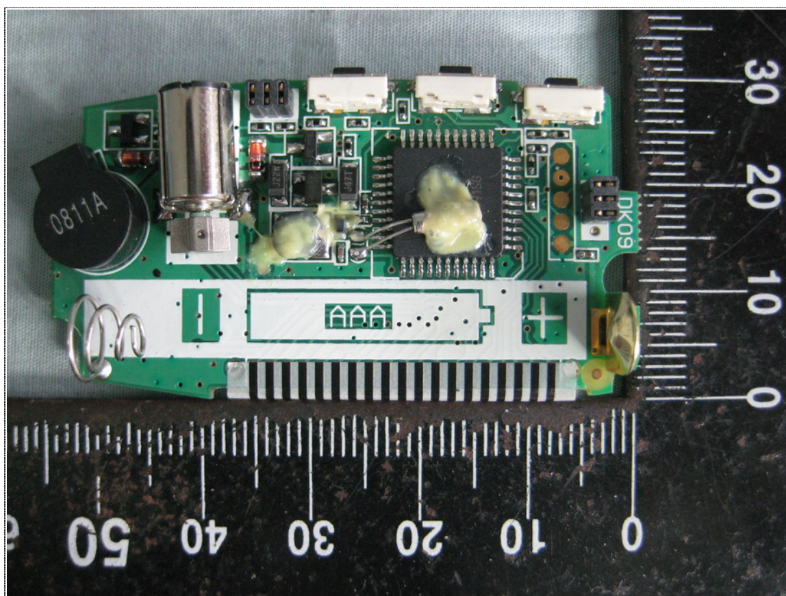
Component View of PCB Board-1
