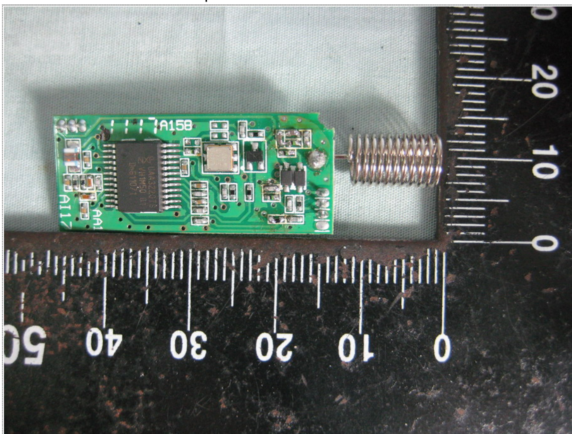
Solder View of PCB Board-2
