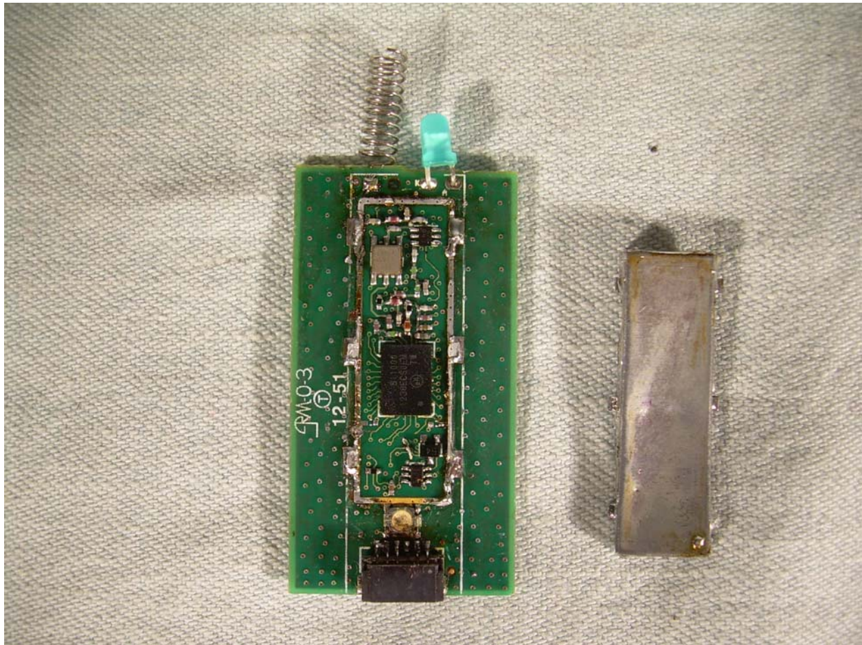
Photograph 6 – View of the Front Side of the PCB with RF Shield Removed
