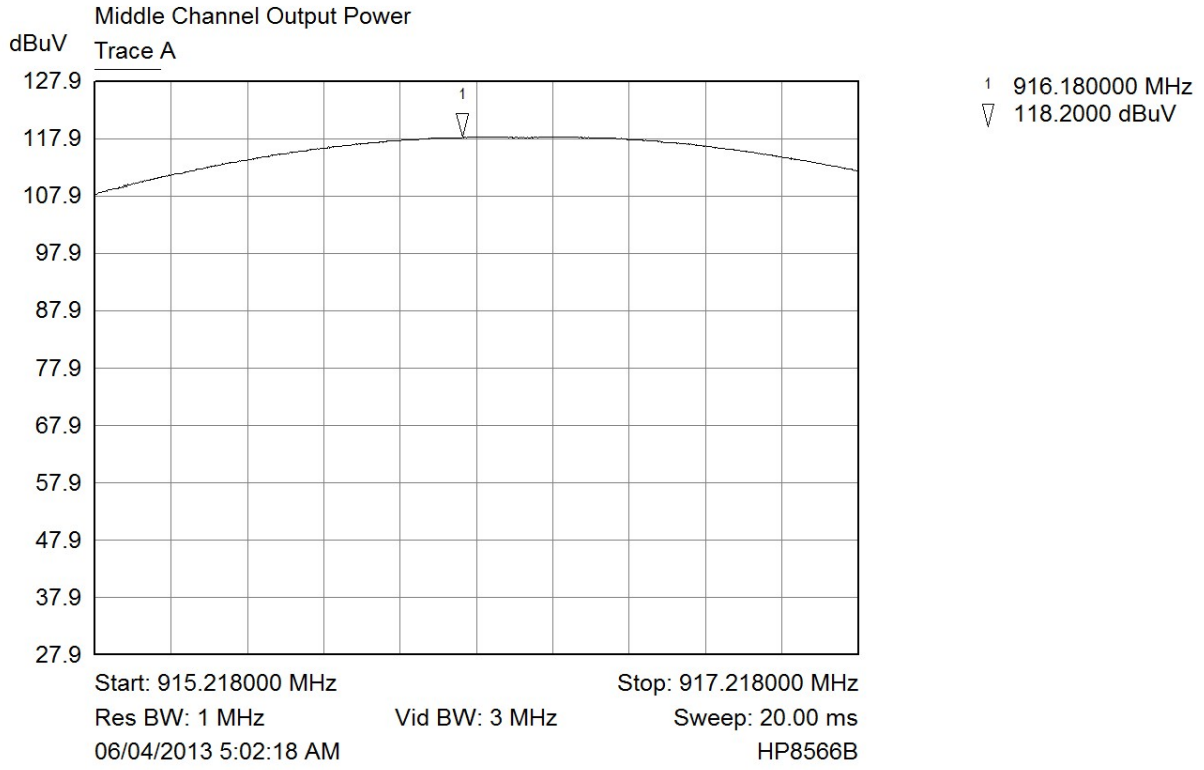
Trace A Middle Channel, Output Power
