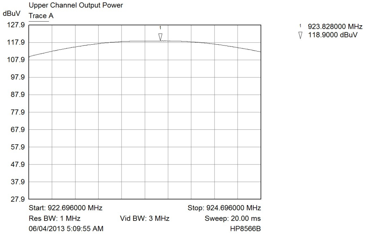
Trace A Upper Channel, Output Power
