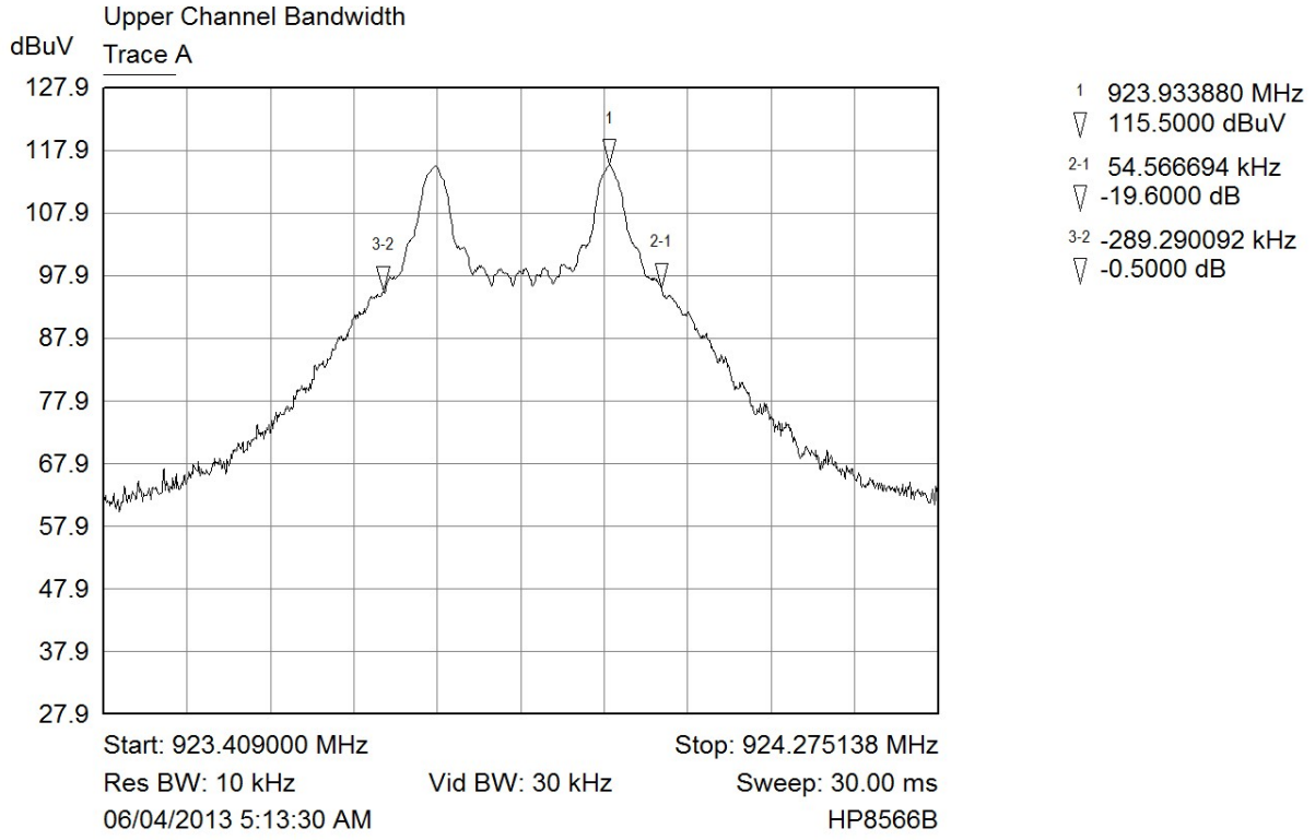
Trace A Upper Channel, Bandwidth
