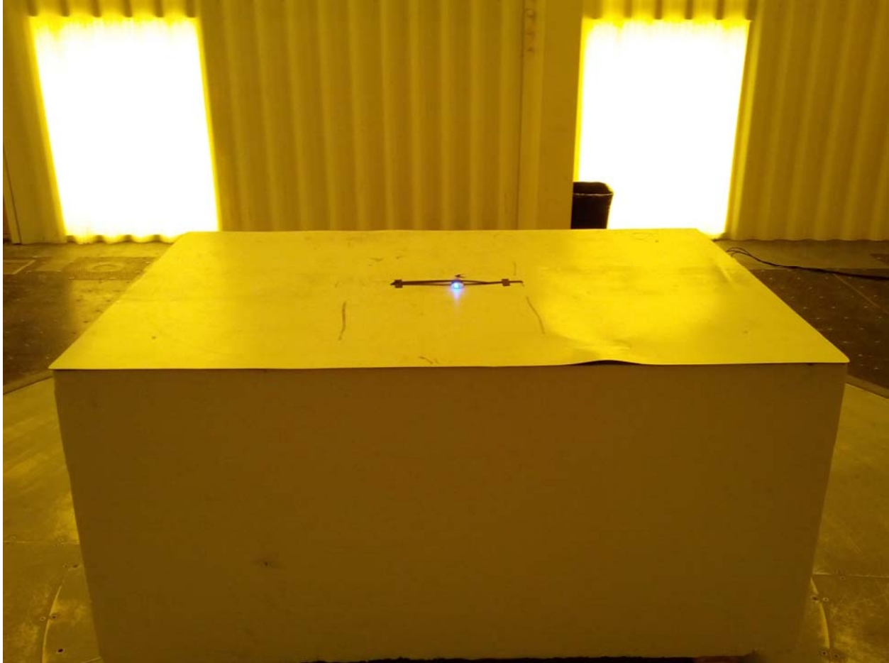
Photograph 1 – Front View Radiated Disturbance Worst Case Configuration (EUT flat)
