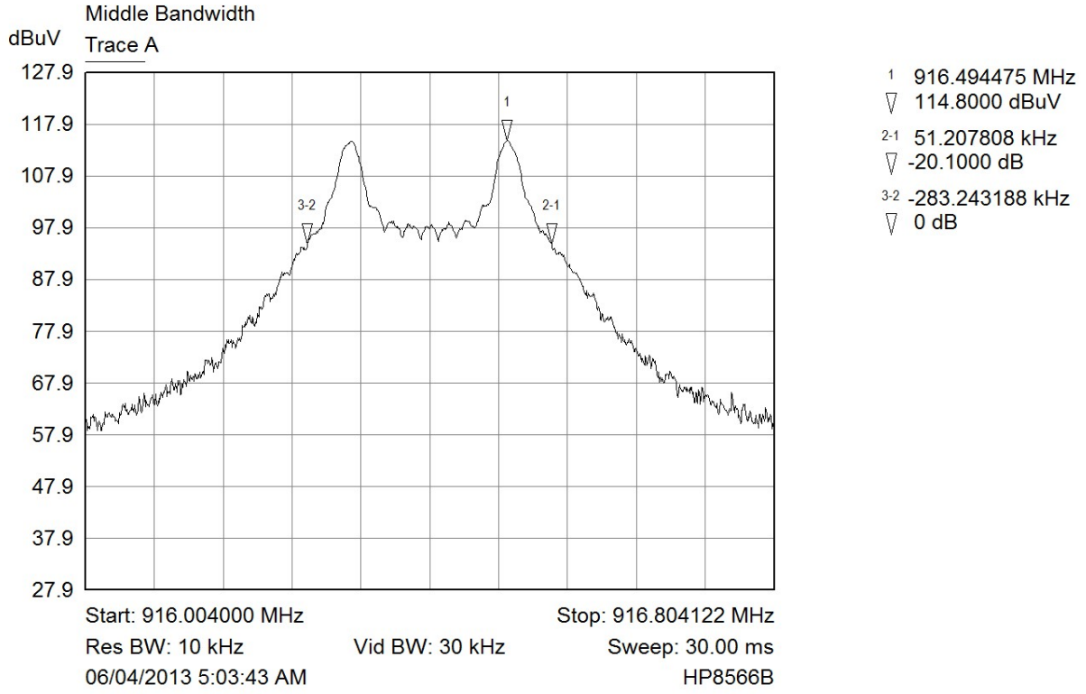
Trace A Middle Channel, Bandwidth
